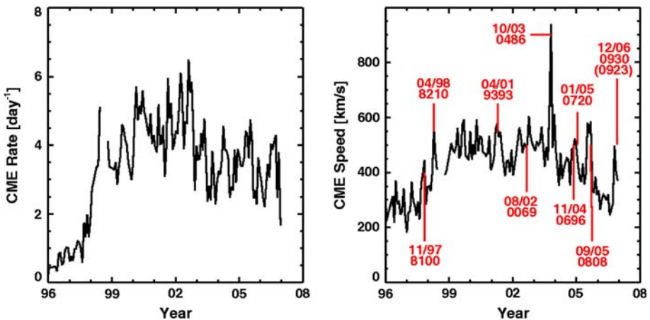
Fig. 9 (left) CME rate (averaged over Carrington Rotation periods) as a function of time for the first 11 years of SOHO observations. The minimum rate is similar to the pre-SOHO values, but the maximum rate is higher by a factor of two. (right) Mean CME speed as a function of time showing that the speed is higher by a factor of 2 during solar maximum phase. The spikes on the CME speed plot are due to some of the super active regions as marked with the month and AR. The mean speed is obtained by averaging the speeds of all CMEs occurring in a given Carrington rotation period
