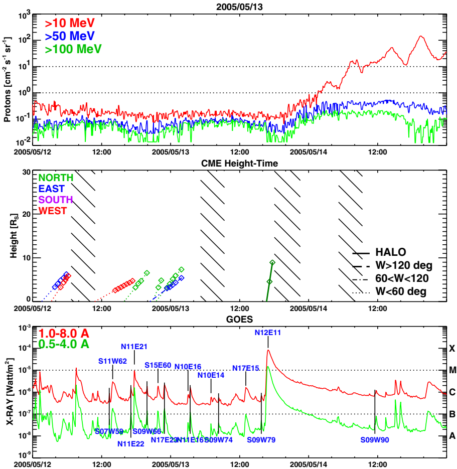
Fig. 4 PHTX plot for 2005 May 13: (top) GOES SEP plots in three energy channels, (middle) CME height-time plots, and (bottom) GOES soft X-ray light curves in two wavelength bands
