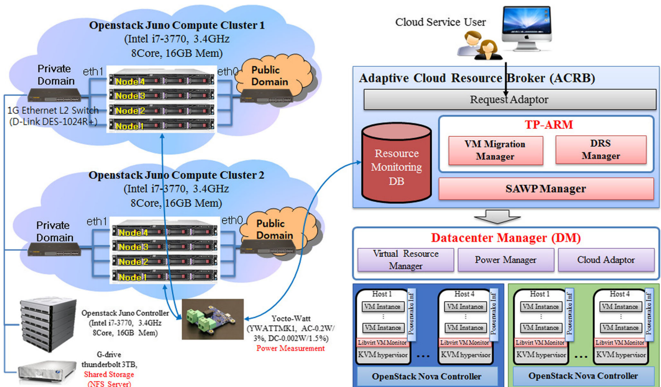
Fig. 6 Experimental Environment
