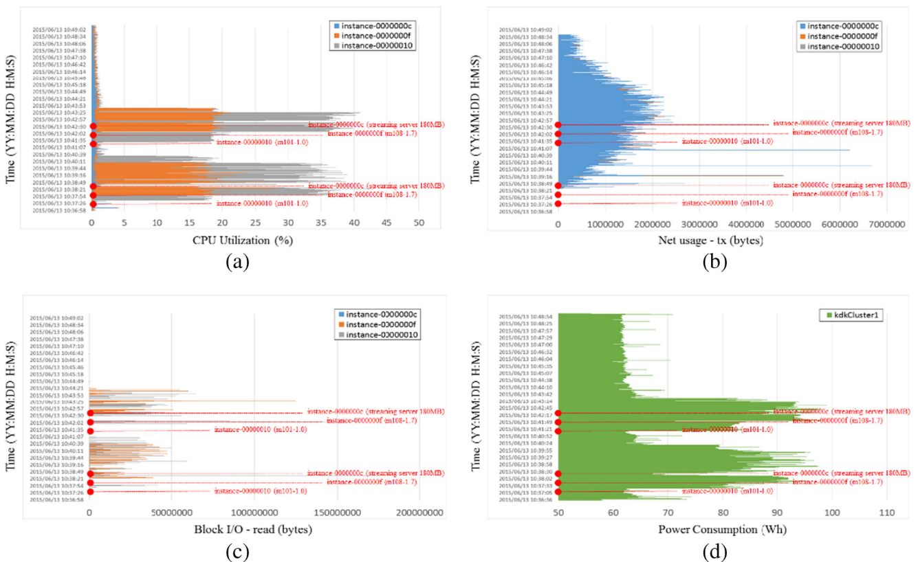
Fig. 8 Librty API monitoring module shows the results of resource utilization of running VM requests in the kdkCluster1 in (a), (b) and (c). Yocto-Watt module [17] was used to measure the power consumption of the kdkCluster1 as shown in (d)
