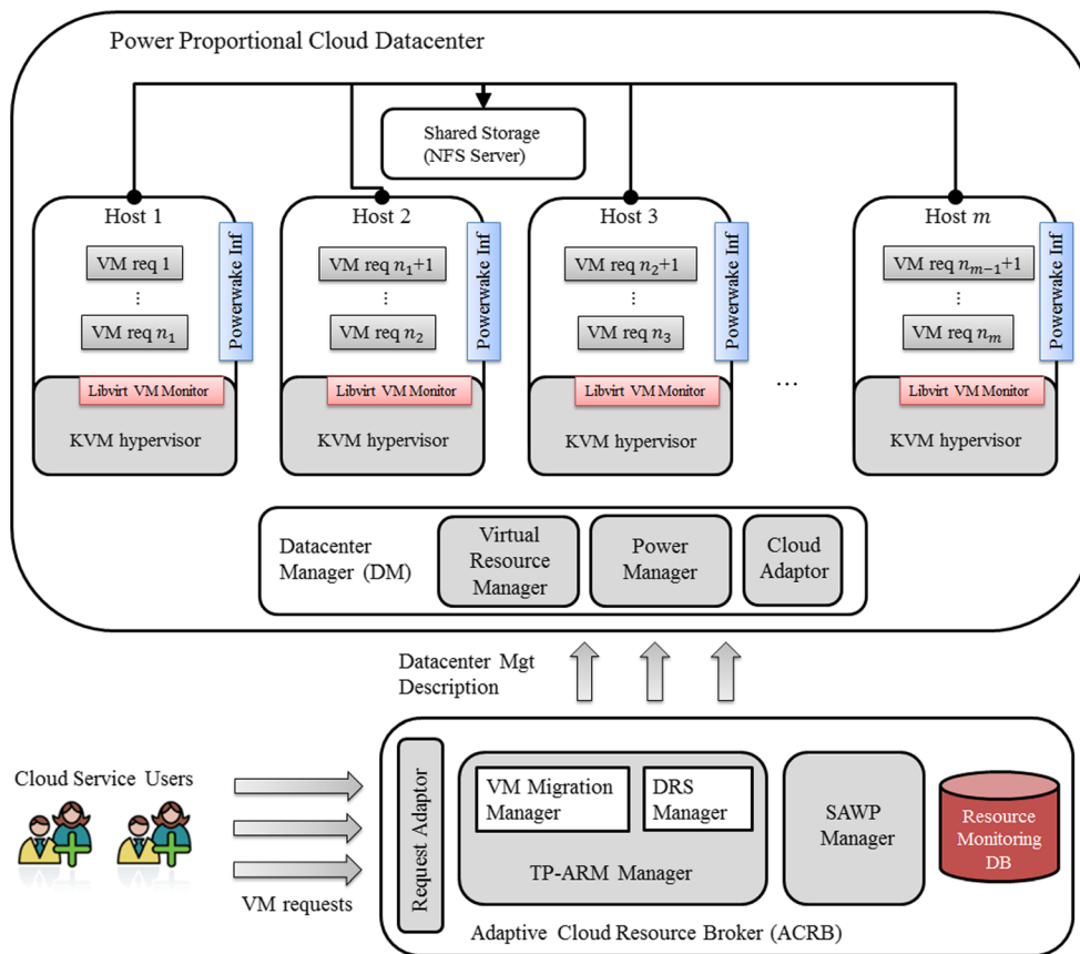
Fig. 1 Adaptive Cloud Resource Brokering (ACRB) system including TP-ARM module and SAWP manager for green cloud datacenters
