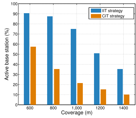
(b) Base station Number for GSM
