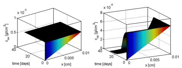
Fig. 13 Spatial and temporal evolution of oxygen concentration in the static culture for c_{ext} = c_{sat} . Initial condition IC2. Left: k_g = k_{g1} . Right: k_g = k_{g2} . In the case of initial condition IC1 we observe a similar behavior of c_{ox} except for a delayed decay
