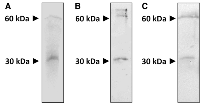
Fig. 1 Western blot analysis of acetylated CACT. Rat liver mitochondrial extract obtained as described in “Materials and methods” section was: a immunoprecipitated by anti-CACT and immunostained with the same antibody; b immunoprecipitated by anti-CACT and immunostained with anti-acetyl-lysine antibody; c immunoprecipitated by anti-acetyl-lysine and immunostained with anti-CACT antibody. The image is representative of at least two independent experiments. Migration of molecular mass standards is indicated by arrows
