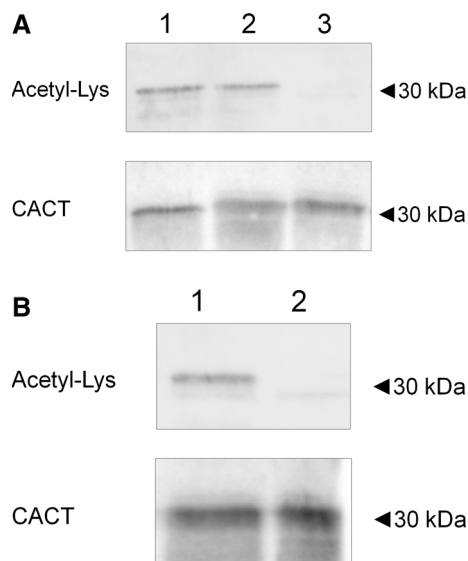
Fig. 2 CACT deacetylation by SIRT3 and localization of acetylated sites. a Protein extract of rat liver mitochondria was incubated at 4 °C, 1 h with no enzyme (lane 1), 3 μg SIRT3 + 5 mM NAD + + 10 mM NAM (lane 2), or 3 μg SIRT3 + 5 mM NAD + (lane 3) and then immunoprecipitated with anti-CACT as described in “Materials and methods” section. Western blot analysis of the samples was performed with anti-acetyl-lysine (upper panel) or with anti-CACT (lower panel) antibodies, in parallel samples. b Intact mitoplasts (lane 1) or mitoplasts solubilized with Triton X-100 (lane 2) were incubated with 3 μg SIRT3 + 5 mM NAD + . Western blot analysis of mitoplast extract immunoprecipitated with anti-CACT and immunostained with anti-acetyl-lysine antibody (upper panel) or with anti-CACT antibody (lower panel), in parallel samples. The image is representative of at least two independent experiments. Migration of molecular mass standards is indicated by arrows
