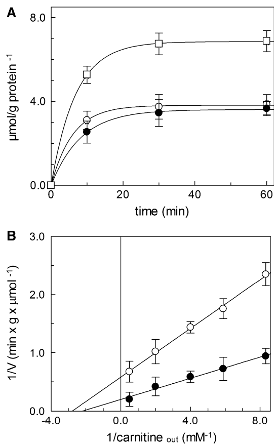
Fig. 5 Effect of CACT acetylation on transport function. a Transport was measured as described in “Materials and methods” section adding measuring [ ^3\text{H} ]carnitine/carnitine antiport in proteoliposomes reconstituted with mitochondrial extract incubated in the absence (white circle) or in the presence of SIRT3 + \text{NAD}^+ + NAM (black circle) or SIRT3 + \text{NAD}^+ (white square). In black circle and white square the reagents were added to the solubilized mitochondria for 1 h at 4 °C before the re constitution procedure. The transport reaction was stopped at the indicated times, as described in “Materials and methods” section. Reported values are mean \pm SD from three experiments. b Kinetic analysis of the effect of SIRT3 on the reconstituted CACT. The [ ^3\text{H} ]carnitine/carnitine antiport rate was measured, as described in “Materials and methods” section, adding [ ^3\text{H} ]carnitine at different concentrations to proteoliposomes reconstituted with mitochondrial extract and containing 15 mM carnitine, in the absence (white circle) or in the presence of (dark circle) SIRT3 + \text{NAD}^+ . In dark circle the reagents were added to the solubilized mitochondria for 1 h at 4 °C before the reconstitution procedure. Experimental data plotted according to Lineweaver–Burk as reciprocal transport rate versus reciprocal carnitine concentrations. Reported values are mean \pm SD from three experiments
