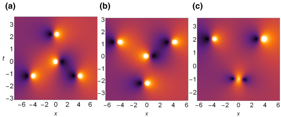
Fig. 9 Three second-order type-III rogue waves. a s_0 = 0, s_1 = 60, r_0 = r_1 = 0 ; b s_0 = 2, s_1 = -60, r_0 = r_1 = 0 ; c s_0 = 2, s_1 = -40, r_0 = 2, r_1 = 0
