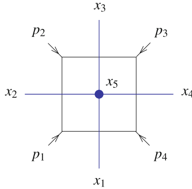
Figure 2. Dual diagram for the one-loop box. The black lines denote the original momentum space loop integral. The propagators can equivalently be represented as scalar propagators in the dual space, denoted by the blue lines .
