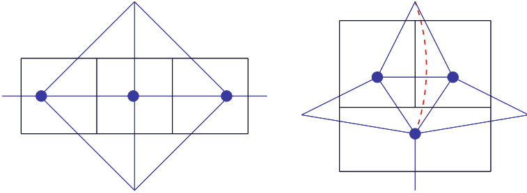
Figure 3. Dual diagrams for the three-loop box and for the ‘tennis court’ with its numerator denoted by the dashed line corresponding to a factor in the numerator of the square distance between the two points.
