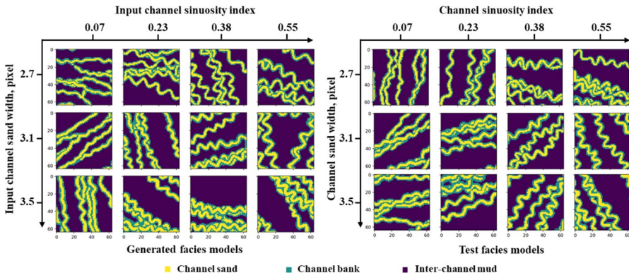
Fig. 9 Generated facies models with various input channel sand width and channel sinuosity index values, and ground truth test facies models with the same channel sand width and channel sinuosity index values. The inter-channel mud facies proportion varies from 0.51 to 0.6
