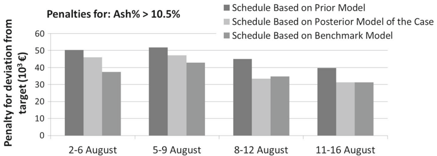
Fig. 10 Cost calculations of deviating from the target quality (ash %)
