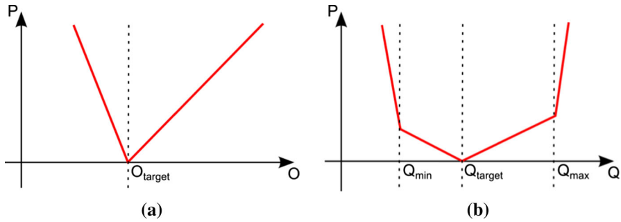
Fig. 3 Penalty functions for not meeting production targets a coal tonnage and b coal quality
