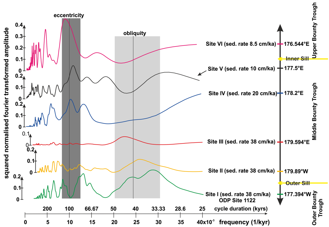
Fig. 4 Spectral analysis of Parasound data from Site I ( lowermost ) to Site VI ( uppermost ). The grey areas indicate the uncertainty ranges for the obliquity cycle (41 kyr cycle) and the eccentricity cycle (125–95 kyr cycle) of the frequency bands
