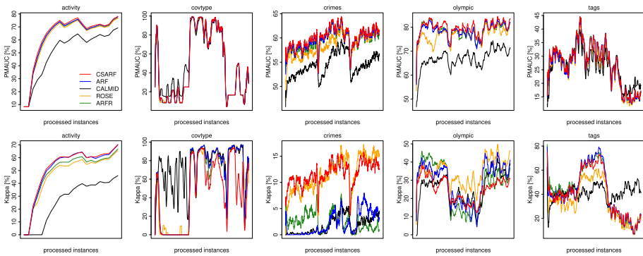
Fig. 41 PMAUC and Kappa on semi-synthetic multi-class imbalanced datasets
