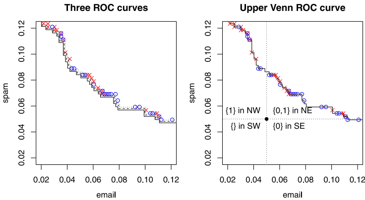
Fig. 11 Left panel: the lower left corner of the lower left plot of Fig. 2 with the empirical ( solid ), minimax ( dashed ), and Laplace ( dotted ) ROC curves. Right panel: the lower left corner of the lower left plot of Fig. 2 with the upper Venn ROC curve and the partition of the plane corresponding to the label conditional ICP with significance level 5 %
