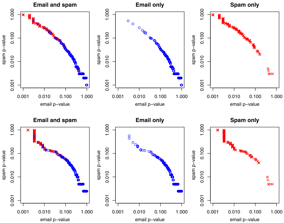
Fig. 3 The analogue of Fig. 2 on the log scale
