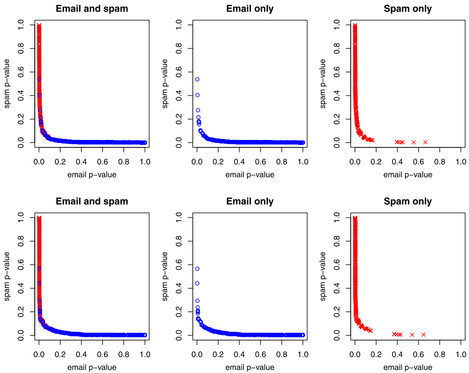
Fig. 2 Scatter plots of the pairs (p^{\text{email}}, p^{\text{spam}}) for all examples in the test set (left plots), for email only (middle), and for spam only (right). Email is shown as (blue) noughts and spam as (red) crosses. The three upper plots are for the ICP and the three lower ones are for the label conditional ICP
