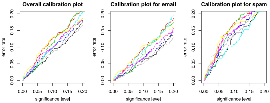
Fig. 5 The lower left corners of the plots in Fig. 4
