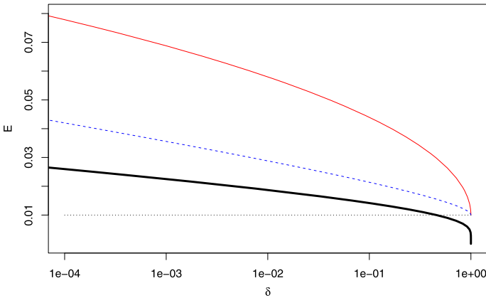
Fig. 10 The analogue of Fig. 8 for \epsilon = 1\%
