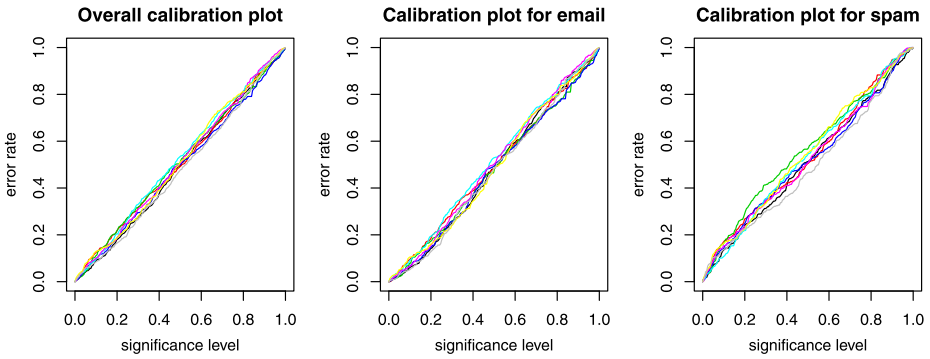
Fig. 4 The calibration plot for the test set overall, the email in the test set, and the spam in the test set (for the first 8 seeds, 0–7)
