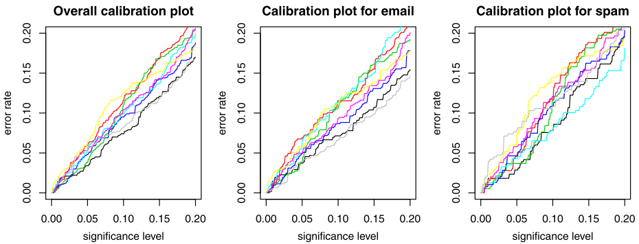
Fig. 6 The analogue of Fig. 5 for the label conditional ICP
