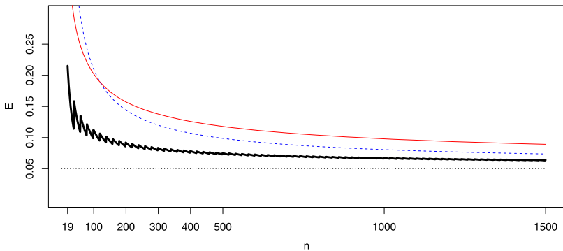
Fig. 9 The upper bounds on the training conditional probability of error vs \delta in the same format as in Fig. 8, except that now \delta is fixed at 1 % and n ranges between 19 (the smallest value giving non-trivial prediction sets) and 1500; as before, \epsilon = 5\%
