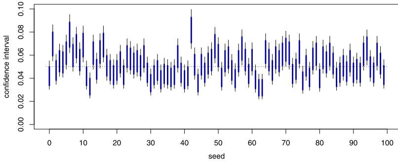
Fig. 7 Confidence intervals for training conditional error probabilities: 95 % shown as thin lines (in black) and 80 % shown as thick lines (perhaps in blue). The 5 % significance level is shown as the horizontal dotted black line
