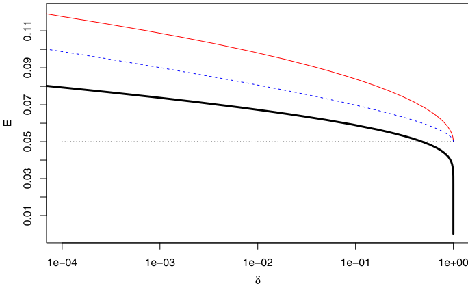
Fig. 8 The upper bounds on the training conditional probability of error vs \delta given by Theorem 1(a) (the thick black line ), Corollary 1(a) (the thin solid line , perhaps shown in red), and Corollary 2(a) (the thin dashed line , perhaps shown in blue), where \epsilon = 5\% and n = 999
