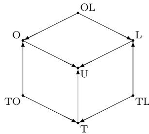
Fig. 1 Eight notions of conditional validity. The visible vertices of the cube are U (unconditional), T (training conditional), O (object conditional), L (label conditional), OL (example conditional), TL (training and label conditional), TO (training and object conditional). The invisible vertex is TOL (and corresponds to conditioning on everything)
