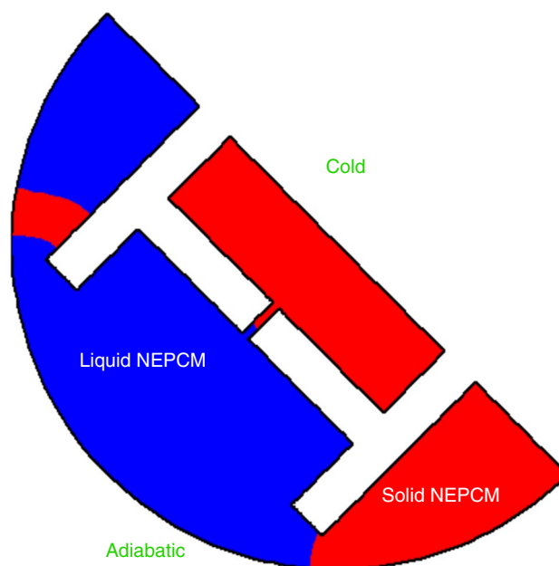
Fig. 1 Freezing within curved tank
