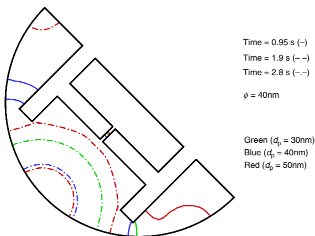
Fig. 8 Greater d_p and progress of ice front
