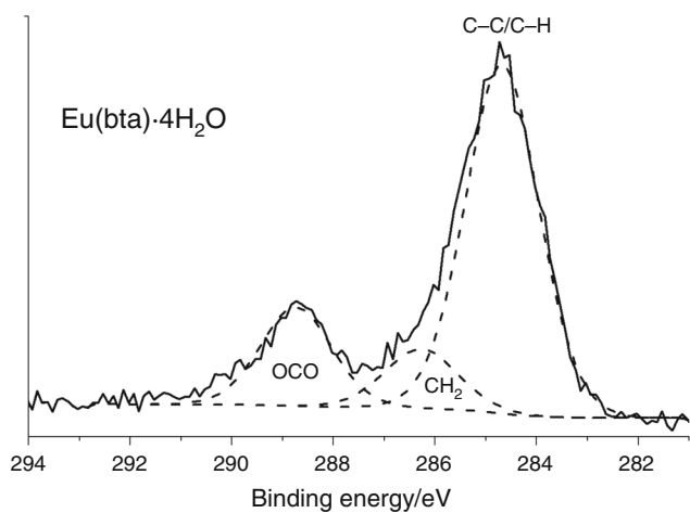
Fig. 8 C1s and O1s spectra of H_3bta and Eu(bta)·4H_2O
