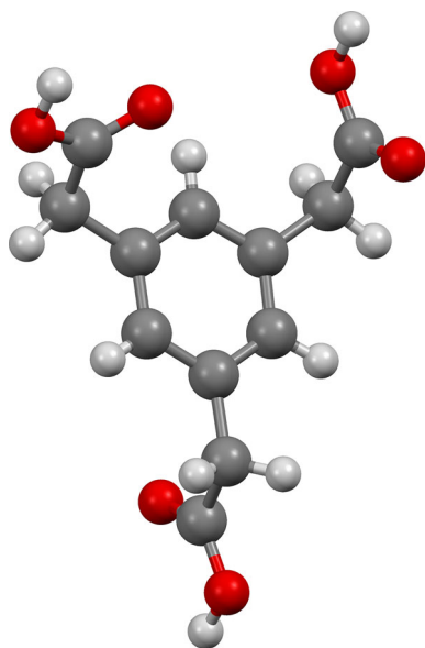
Scheme 2 Molecular structure of neutral H_3bta [23]
