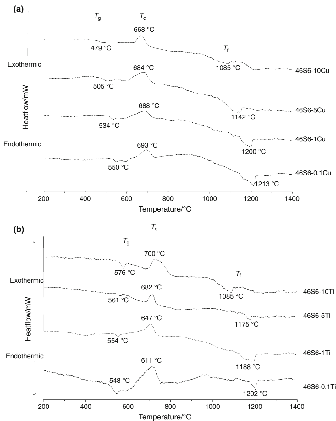
Fig. 3 a Thermal curves of Cu-doped glasses, b thermal curves of Ti-doped glasses
