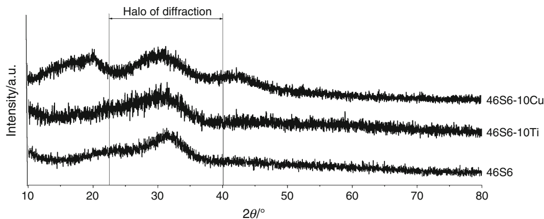
Fig. 1 Diffractograms of pure and doped glasses
