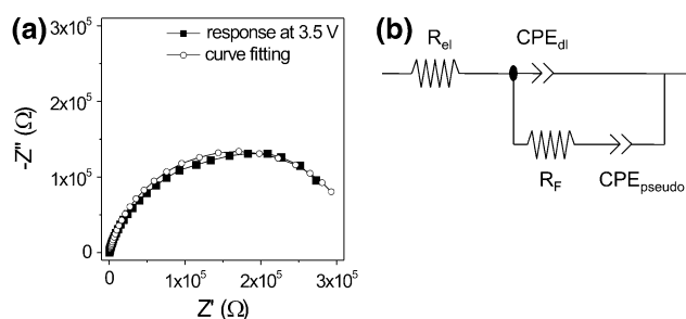
Fig. 4 Electrochemical impedance spectroscopy for mesoporous CeO 2 films. a Nyquist representation at 3.5 V when Ce is fully oxidized. b Equivalent circuit model for mesoporous CeO 2 films. Reprinted with permission [8]
