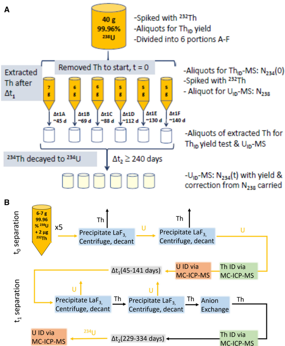
Fig. 1 Schematic overview a of ^{234}\text{Th} ingrowth experiment that was designed as an independent measurement of \lambda_{\text{U-}^{238}} , with the t_0 and t_1 chemical separations summarized in b . Six aliquots of 99.96% ^{238}\text{U} were chemically-purified to establish the beginning time ( t = 0 ) and were quantified by uranium isotope dilution–mass spectrometry ( \text{U}_{\text{ID}}\text{-MS} ) using the ^{233}\text{U}/^{236}\text{U} double-spike from the Institute for Reference Materials and Measurements (IRMM-3636, [15]) before decaying for different ingrowth periods ( \Delta t_1 ). Ingrown thorium was extracted and purified after \Delta t_1 , and small aliquots were removed for yield measurements via thorium isotope dilution mass spectrometry using a ^{229}\text{Th} spike ( \text{Th}_{\text{ID}}\text{-MS} ). The bulk extracted Th aliquots decayed to ^{234}\text{U} over > 10 ^{234}\text{Th} half-lives ( \Delta t_2 ), then measured by \text{U}_{\text{ID}}\text{-MS} . The number of ^{234}\text{U} atoms measured in each aliquot after \Delta t_2 reveals the number of ^{238}\text{U} atoms that decayed during \Delta t_1
