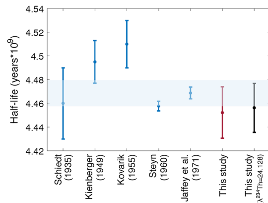
Fig. 5 Uranium-238 half-life determined in the present study using the currently evaluated \lambda_{234\text{Th}} (red) or a new weighted average \lambda_{234\text{Th}} (black) alongside previously reported values from \alpha -counting experiments (blue), with the first author and year listed, adapted from (Schön et al. 2003). Of these, only our measurement, Kienberger 1949, and Jaffey 1971 were direct measurements of enriched ^{238}\text{U} , the rest are correlated with assumed natural uranium isotope ratios. All vertical bars represent the stated uncertainty ( k = 2 ), and the evaluated uncertainty ( k = 2 ) envelope (from Villa et al. 2016) is shaded light blue
