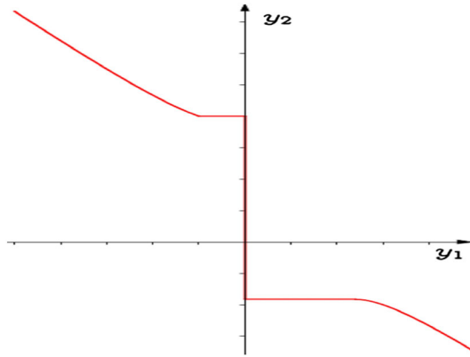
Fig. 1 Representation of the set (f + i_C + (1, \frac{1}{2}) \circ g)^*(0, -1)
