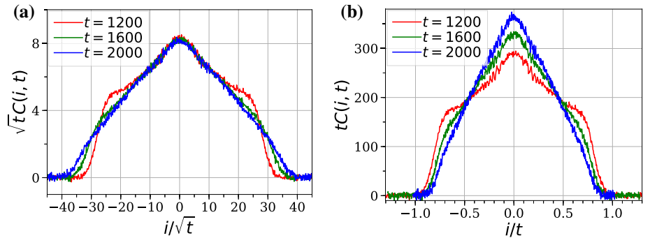
Fig. 9 Energy correlations for system size N = 4096 at high temperature T = 20 with Toda parameters ( a = b = 1, \nu = 2, \zeta = 2 ) and averaged over \approx 10^6 data points with a diffusive scaling of energy correlations, b ballistic scaling for energy correlations. We see that there is a better collapse of data with diffusive scaling though we are not yet in the fully diffusive limit. Also note the highly non-Gaussian form
