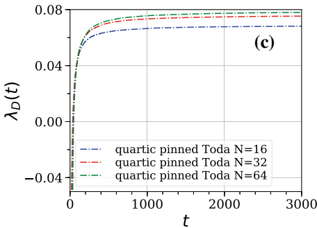
Fig. 11 The time-dependent quantity \lambda(t) as defined in Eq. 2.10 is plotted as a function of time for different models. At large times, this quantity gives the largest Lyapunov exponent in the system. a \lambda(t) for the quadratically pinned Toda chain ( a = b = 1, \nu = 2, z = 2, ) for both low temperatures (dashed lines: T = 1 ) and high temperatures (solid line: T = 20 ). At large times both converge to a finite positive value and this shows that the system has positive Lyapunov exponent and hence is non-integrable. There is a weak dependence of the Lyapunov exponent with system size (shown in different colours) for small systems, b \lambda(t) for the pinned harmonic chain and the unpinned Toda chain ( a = b = 1, \nu = 0 ) which are both integrable. In both the cases, \lambda(t) \sim 1/t for large t , as is seen clearly in the inset. c \lambda(t) for the quartic pinned Toda ( a = b = 1, \nu = 2, z = 4, T = 1 ). Here the Lyapunov exponent is positive and large even at low temperatures
