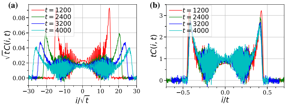
Fig. 6 Energy correlations for system size N = 4096 at low temperature T = 1 with Toda parameters ( a = b = 1, v = 2, z = 2 ) and averaged over \approx 10^6 data points with a diffusive scaling of energy correlations. b Ballistic scaling for energy correlations. We see that at very large times, the equilibrium correlations are still very close to ballistic scaling, although this is not perfect, which is not surprising since we have seen in the non-equilibrium simulations that we start seeing significant gradient already at this system size
