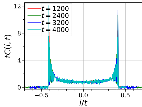
Fig. 6 Energy correlations for system size N = 4096 at low temperature T = 1 with Toda parameters ( a = b = 1, v = 2, z = 2 ) and averaged over \approx 10^6 data points with a diffusive scaling of energy correlations. b Ballistic scaling for energy correlations. We see that at very large times, the equilibrium correlations are still very close to ballistic scaling, although this is not perfect, which is not surprising since we have seen in the non-equilibrium simulations that we start seeing significant gradient already at this system size
