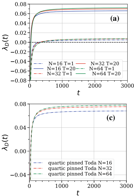
Fig. 11 The time-dependent quantity \lambda(t) as defined in Eq. 2.10 is plotted as a function of time for different models. At large times, this quantity gives the largest Lyapunov exponent in the system. a \lambda(t) for the quadratically pinned Toda chain ( a = b = 1, \nu = 2, z = 2, ) for both low temperatures (dashed lines: T = 1 ) and high temperatures (solid line: T = 20 ). At large times both converge to a finite positive value and this shows that the system has positive Lyapunov exponent and hence is non-integrable. There is a weak dependence of the Lyapunov exponent with system size (shown in different colours) for small systems, b \lambda(t) for the pinned harmonic chain and the unpinned Toda chain ( a = b = 1, \nu = 0 ) which are both integrable. In both the cases, \lambda(t) \sim 1/t for large t , as is seen clearly in the inset. c \lambda(t) for the quartic pinned Toda ( a = b = 1, \nu = 2, z = 4, T = 1 ). Here the Lyapunov exponent is positive and large even at low temperatures
