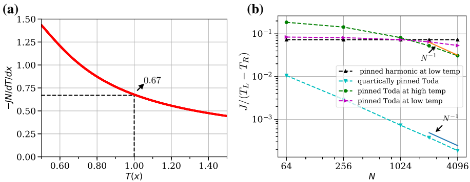
Fig. 5 a The thermal conductivity ( \kappa = JN/\frac{dT}{dx} ) plotted as a function of temperature [ T(x) \in (0.5, 1.5) ] for the quartic pinned Toda chain for system size N = 4096 . The thermal conductivity is a function of temperature in this system. The thermal conductivity at T = 1 can be seen to be \kappa \approx 0.67 . b Current scaling with system size for various setups
