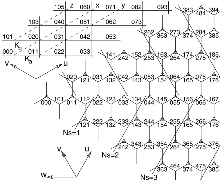
Fig. 4 A \pi/3 section of the triangular/honeycomb lattice. Small triangles mark the triangular and even honeycomb lattice sites. Numbers are the i, j indices of the g and g^* correlation functions. Lines labelled by N_s are the boundaries of the “shells” described in the text. The inset shows the g and g^* labelling of sites on the anisotropic square lattice. Vectors are the directions of the rapidity lines on the two lattices. Dashed lines labelled x, y and z indicate the diagonal and near diagonal elements calculated by the Witte recursion relations described in Sect. 3.1. Note that the two lowest rows on the square correspond exactly to two rows on the triangular lattice. Sites equivalent by symmetry have identical indices
