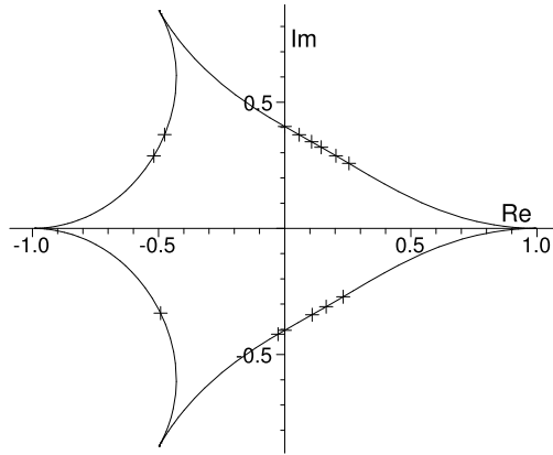
Fig. 5 The conjectured natural boundary in the complex (cube root) nome \bar{q} -plane for the Ising model on the triangular lattice. The real axis cusps are the points u = \pm 1/3 ; the other two are u = -1 + i0^\pm . The right side arcs are defined by |k_{tr}| = 1 and u = (-1 + 2e^{i\phi})/3 , -\pi < \phi < \pi . The left arcs correspond to straight line segments lying on either side of the cuts, -\infty < k_{tr} \leq -1 in k_{tr} and -1 \leq u \leq -1/3 in u . Crosses mark the singularities found in the series analysis described in the text. For clarity, the singularities for T < T_c are shown only in the upper half plane , those for T > T_c in the lower half
