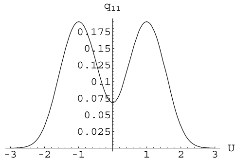
Fig. 13 The function q_{11}(U) = \int P(U, u_1, u_2)u_1^2 du_1 du_2 (modulo an unknown positive constant scaling as T_c - T ) at a generic temperature slightly below T_c = 2.2 for the 4DEA with bimodal interactions, see text. It is always positive as it should since P(U, u_1, u_2) is a distribution
