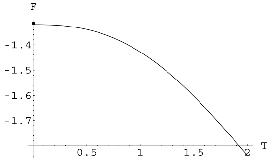
Fig. 4 Free energy vs. Temperature of the paramagnetic solution in the plaquette approximation (solid) for the 2DEA model with Gaussian couplings. The dot at T = 0 corresponds to the value of the ground state energy of the actual model
