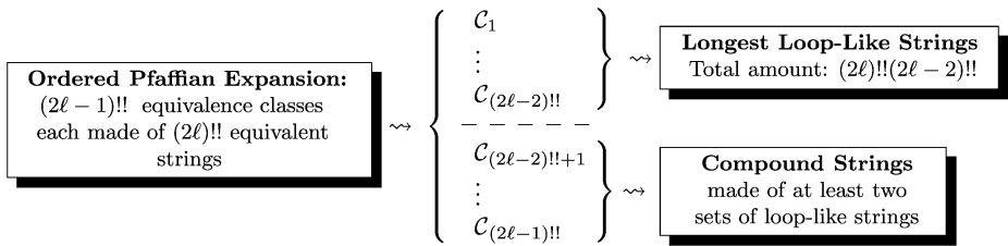
Fig. 3 The (2\ell)! terms, or strings, of an ordered Pfaffian expansion can be assigned to (2\ell - 1)!! equivalence classes \{C_1, \dots, C_{(2\ell-1)!!}\} , each one containing (2\ell)!! equivalent strings (Lemma 5.1). Any given string of the length \ell can be decomposed into a set of loop-like substrings of respective lengths \{\ell_j\} such that \sum_j \ell_j = \ell (Lemma 5.2). The sets consisting of only one loop-like string are called longest loop-like strings ; the sets made of more than one loop-like substring are called compound strings . An amount of longest loop-like strings is counted in Lemma 5.3
