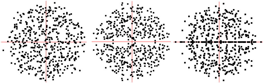
Fig. 1 Numerically simulated distributions of complex eigenvalues in GinUE ( left panel ), GinSE ( middle panel ), and GinOE ( right panel ). Three different eigenvalue patterns are clearly observed. Eigenvalues are scattered almost uniformly in GinUE, depleted from the real axis in GinSE, and accumulated along the real axis in GinOE
