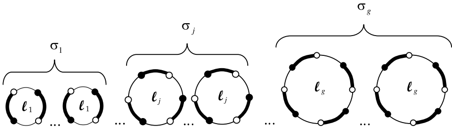
Fig. 6 A diagrammatic representation of a compound string belonging to the topology class \lambda = (\ell_1^{\sigma_1}, \dots, \ell_g^{\sigma_g}) with \sum_{j=1}^g \ell_j \sigma_j = \ell and \sum_{j=1}^g \sigma_j = r . Here, g denotes the number of inequivalent parts of the partition \lambda whilst r equals the total number of loops
