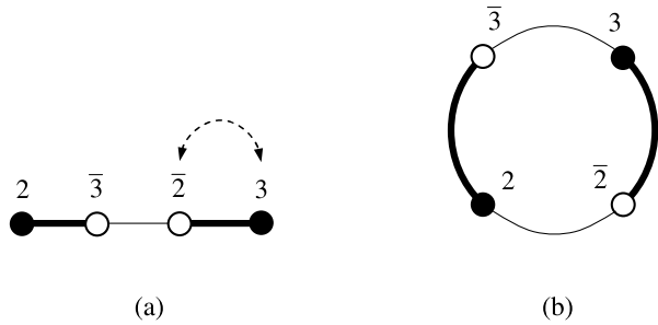
Fig. 4 Graphic explanation of the notion “loop-like substring”. (a) The substring (\bar{2}\bar{3})(\bar{2}\bar{3}) can be transformed into the form of an adjacent substring (in the sense of Definition 5.7) by flipping arguments in the second kernel, (\bar{2}\bar{3}) \mapsto (3\bar{2}) . (b) The emerging adjacent substring (\bar{2}\bar{3})(3\bar{2}) can clearly be depicted in the form of a loop by gluing the arguments 2 and \bar{2} together
