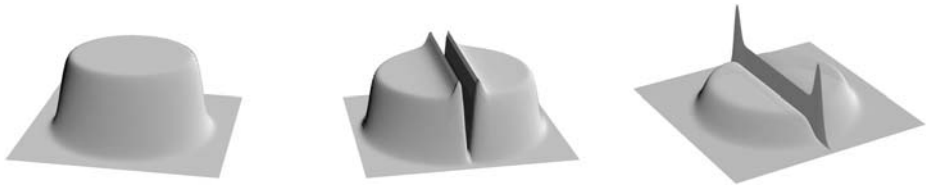
Fig. 2 Profiles of eigenlevel densities R_1^{(\beta)}(z; n) , plotted as functions of the complex energy z = x + iy for n fixed, show a nearly uniform eigenlevel distribution in GinUE (left panel), a depletion of eigenvalues along the real axis in GinSE as exemplified by the density drop at y = 0 (middle panel), and accumulation of real eigenvalues in GinOE displayed as a wall at y = 0 (right panel); the wall height imitates the density of real eigenvalues
