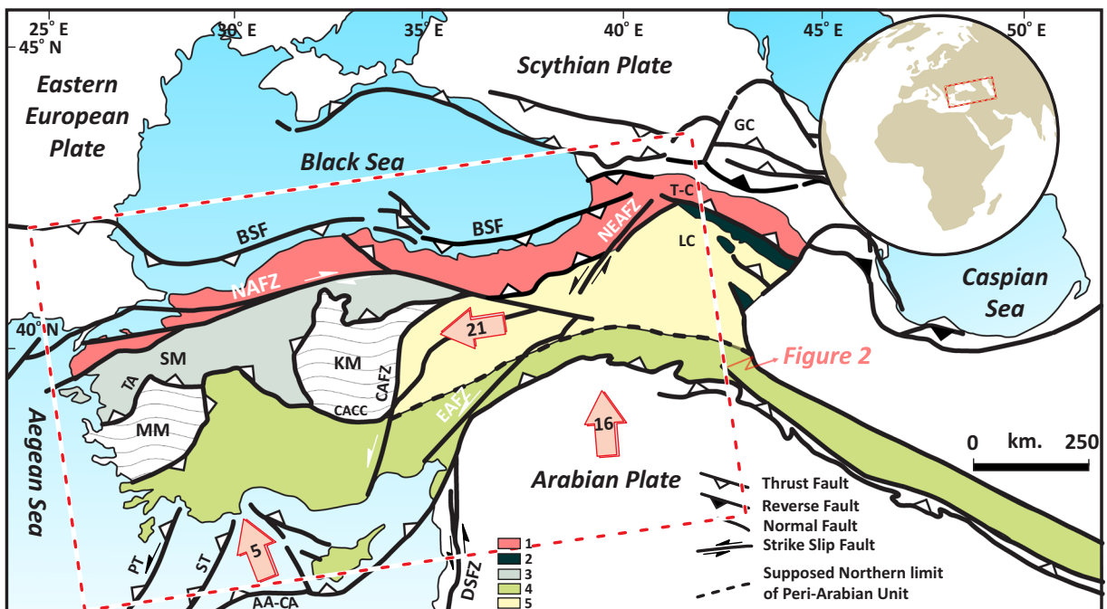
Fig. 1 Brief amalgamated geologic and tectonic map of the Anatolia–Caucasus region, after Sosson et al. (2016) and Hässig et al. (2016) with modifications. NAFZ, North Anatolian Fault Zone; CAFZ, Central Anatolian Fault Zone; EAFZ, East Anatolian Fault Zone; NEAFZ, Northeast Anatolian Fault Zone; BSF, Black Sea Fault; DSFZ, Dead Sea Fault Zone; PT, Plino Trench; ST, Strabo Trench; AA-CP, Aegean–Cyprus Arc; GC, Greater Caucasus; LC, Lesser Caucasus; T-C, Trans Caucasus; KM, Kirsehir Massif; MM, Menderes Massif; SM, Sakarya Massif;
