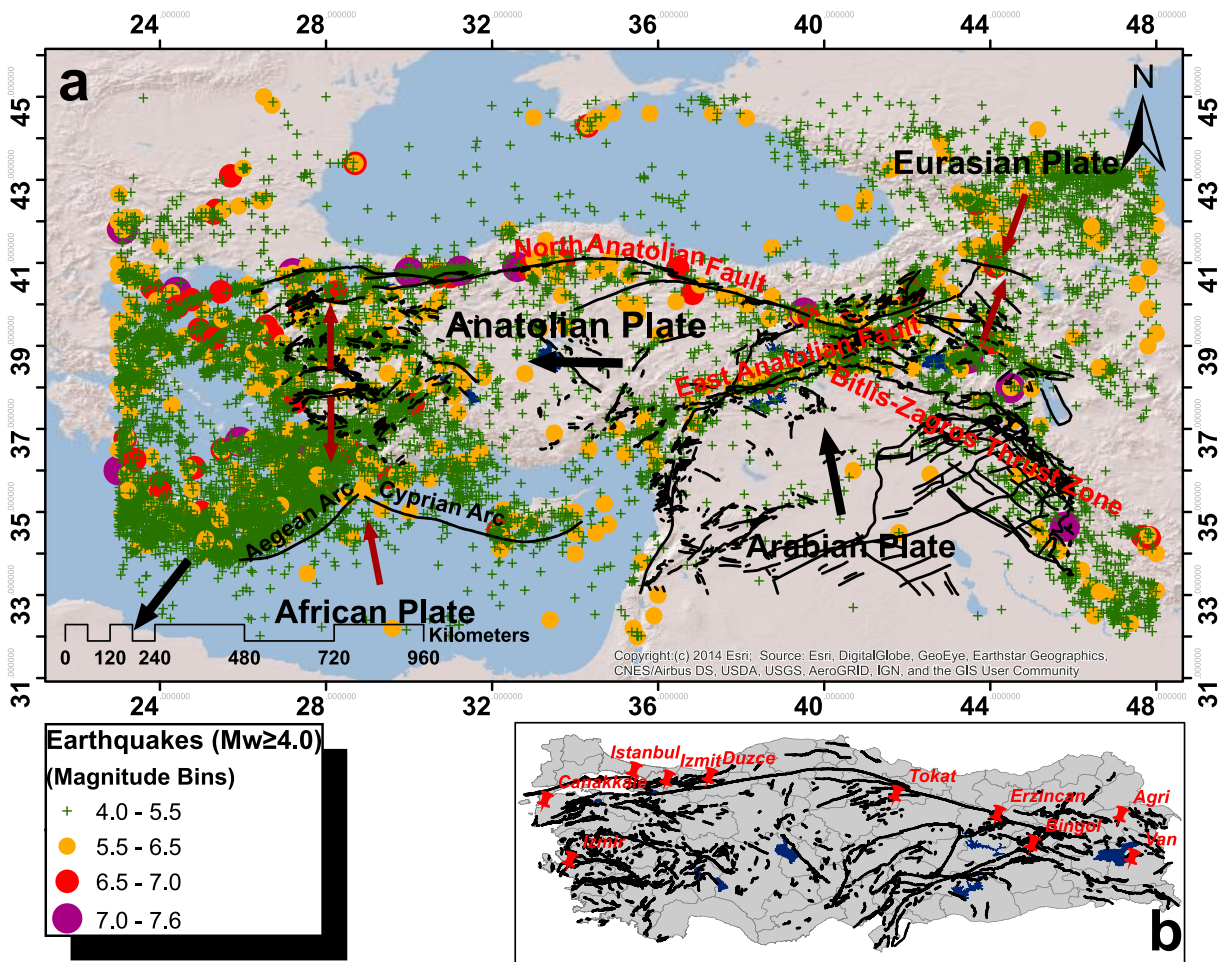
Fig. 2 a Illustrative map of the brief seismotectonic setup with earthquakes occurred between 1900 and 2018 in and around Turkey used in this study. b Site location map of the surveyed ten earthquake-prone cities of Turkey in this study
