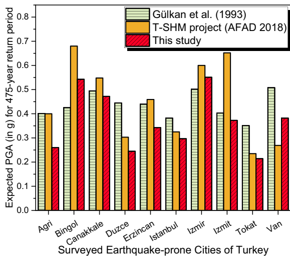
Fig. 8 Comparison of the maximum expected PGA (upon 90% quantile, in g) for ten earthquake-prone cities of Turkey (all of the PGA values are calculated by taking into account the reference-rock site condition ( V_{S30} = 760 m/s) and a return period of 475 years)
