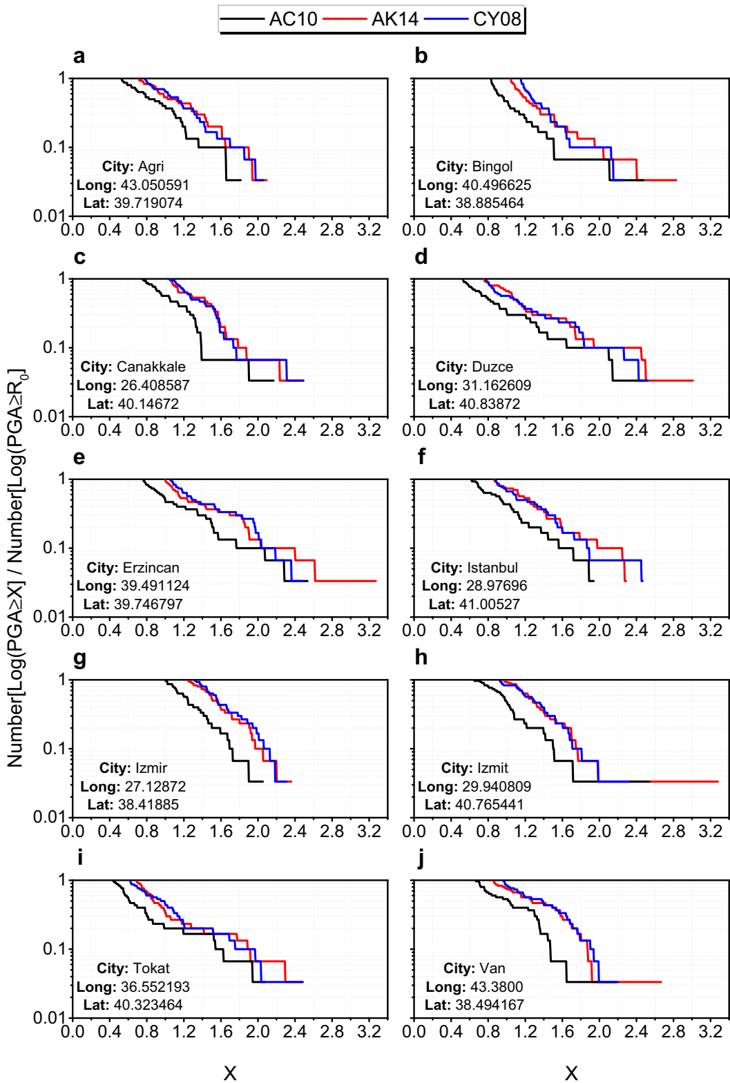
Fig. 6 a–j Empirical tail probability functions of PGA distributions (for 475-year RP and V_{S30} = 760 m/s, in g) for ten earthquake-prone city centers concerning AK14, AC10, and CY08 respectively
