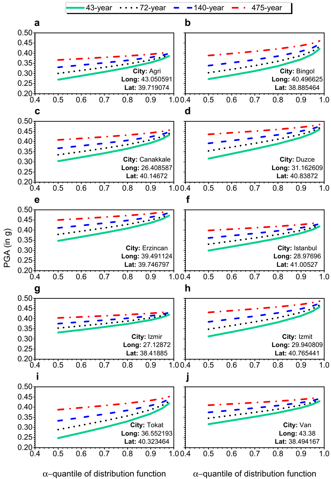
Fig. 7 a–j The quantiles of the distribution function of estimated PGA values (in g, upon 90% quantile) for ten earthquake-prone cities of Turkey (the curves represent the expected PGA values depending on 43, 72, 140, and 475 years of return period and V_{S30} = 760 m/s)
