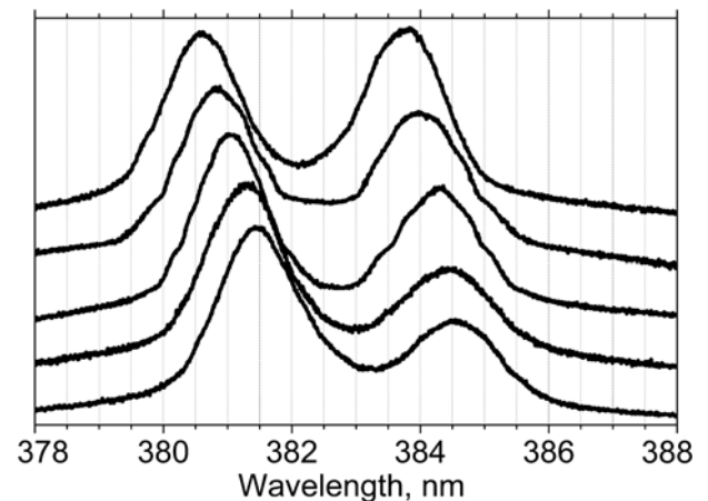
Fig. 3. Laser spectra at different places under fixed pumping level (sample 1).
