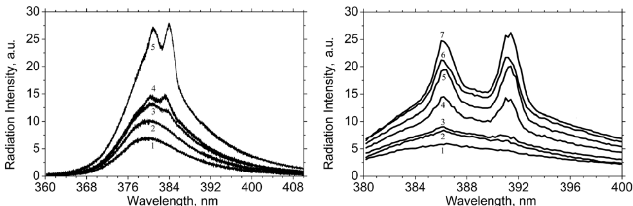
Fig. 4. Spectra of microtowers under different pumping levels 2.6 (1), 4.3 (2), 5.0 (3), 9.0 (4), and 13.1 \text{mJ}\cdot\text{cm}^{-2} (5) for sample 1 (left) and 4.2 (1), 6.4 (2), 8.1 (3), 11.4 (4), 15.5 (5), 19.1 (6), and 23.7 \text{mJ}\cdot\text{cm}^{-2} (7) for sample 2 (right).
