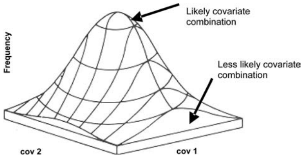
Fig. 1. Illustration of multivariate normal distribution for two covariates (cov1 and cov2). Covariate combinations that occur naturally in the target population have a high probability of being selected by the covariate distribution model, whereas unrealistic or physiologically impossible combinations are selected with lower frequency.
