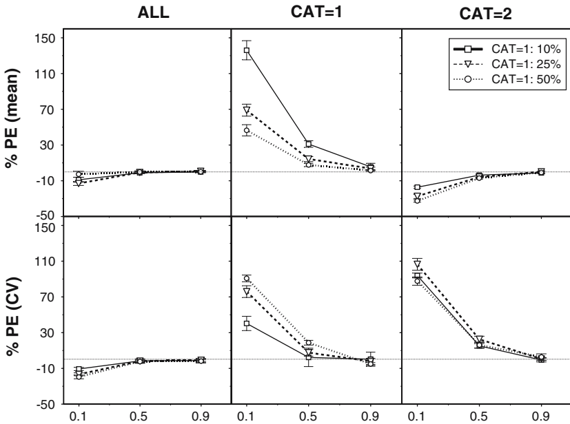
Fig. 7. Simulated Data: Percent error in mean (top row) and CV (bottom row) of CONT1 for the values generated by the Continuous method, as a function of mode ratio and % (CAT=1).
