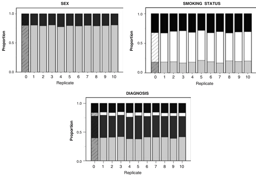
Fig. 3. Real Data Example: Proportion of patients in each level for the three categorical covariates. The leftmost bar in each plot represents the target population data ( n = 467 ). Each additional bar represents one replicate of 1000 patients, generated using the Continuous method. The varying bar colors represent the proportion of subjects in each category.
