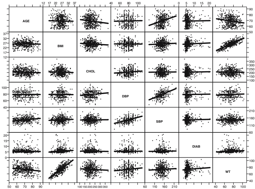
Fig. 10. Scatterplot matrix for observed continuous covariates in real data set. Lines represent Loess smooths of the individual plots, and indicate that the relationships between the covariates are relatively linear; thus, it is appropriate to enter all covariates into the MVND.
