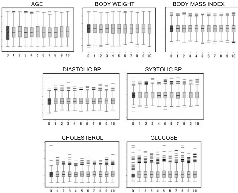
Fig. 4. Real Data Example: Box and whisker plot showing the distribution of values for the continuous covariates. The leftmost box in each plot represents the target population data ( n = 467 ). Each additional box represents one replicate of 1000 patients, generated using the Continuous method. The boxes contain the 25th to 75th percentiles, the horizontal bar represents the median value, the whiskers represent the 10th to 90th percentiles, and the lines outside the whiskers represent outliers.
