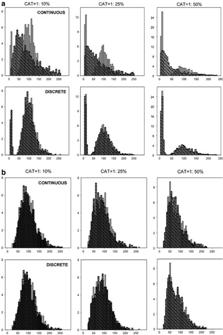
Fig. 6. (a) Simulated Data: Population distribution of CONT1 for MR = 0.1. The target population covariate data (gray bars) is overlaid with the Continuous method results (top) and Discrete method results (bottom), shown as transparent bars. Only the scenarios for correlation = 0 between CONT1 and CONT2 are shown, but the plots for correlations of 0.45 and 0.9 look similar. (b) Simulated Data: Population distribution of CONT1 for MR = 0.5. (c) Simulated Data: Population distribution of CONT1 for MR = 0.9.
