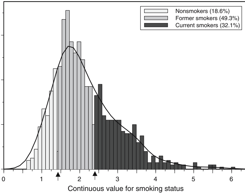
Fig. 2. Illustration of the calculation of discrete values for smoking status with three possible values (nonsmoker, former smoker, current smoker). The mean and standard deviation define the log-normal probability distribution of smoking status in the empirical distribution, as if it was a continuous covariate. The histogram is derived from an empirical distribution used to estimate the continuous distribution parameters. The cumulative probability ( P ) corresponds to the area under the probability distribution curve (solid line). The CrVs are indicated by arrows on the x -axis.
