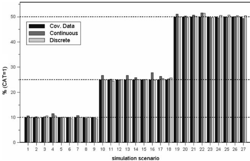
Fig. 5. Simulated Data: Bar chart showing the percentage of patients in the subgroup (CAT=1) for the target population covariate data and the covariate data generated by the Continuous and Discrete methods. There should be 10, 25, and 50% in the (CAT=1) subgroup, respectively, for each set of 9 scenarios.
