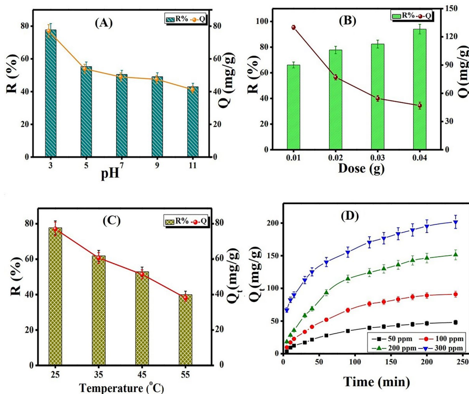
Fig. 7 Effect of A pH, B Dose, C Temperature, and D Initial concentration on the capacity of the CR adsorption onto Fe25/MOF-5@CTS composite film
