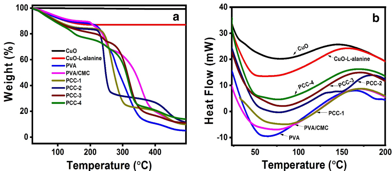
Fig. 7 TGA (a) and DSC (b) curves of prepared PVA, PVA/CMC and NC films
