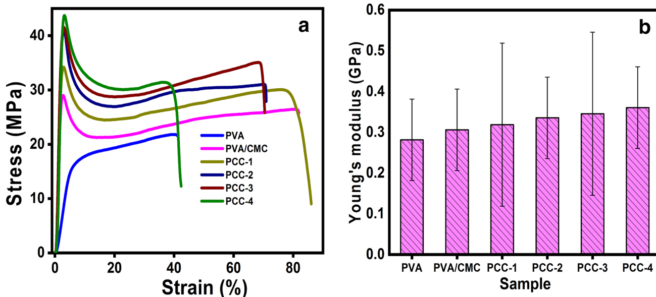
Fig. 6 Breaking stress and elongation at break (a) and Young's modulus (b) of PVA, PVA/CMC and NC film (mean \pm SD, n=3 )
