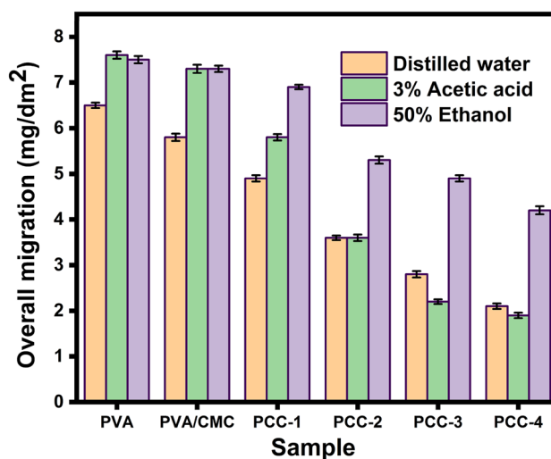
Fig. 9 Overall migration rate (food compatibility) of PVA, PVA/CMC and NC films (mean \pm SD, n = 3)
