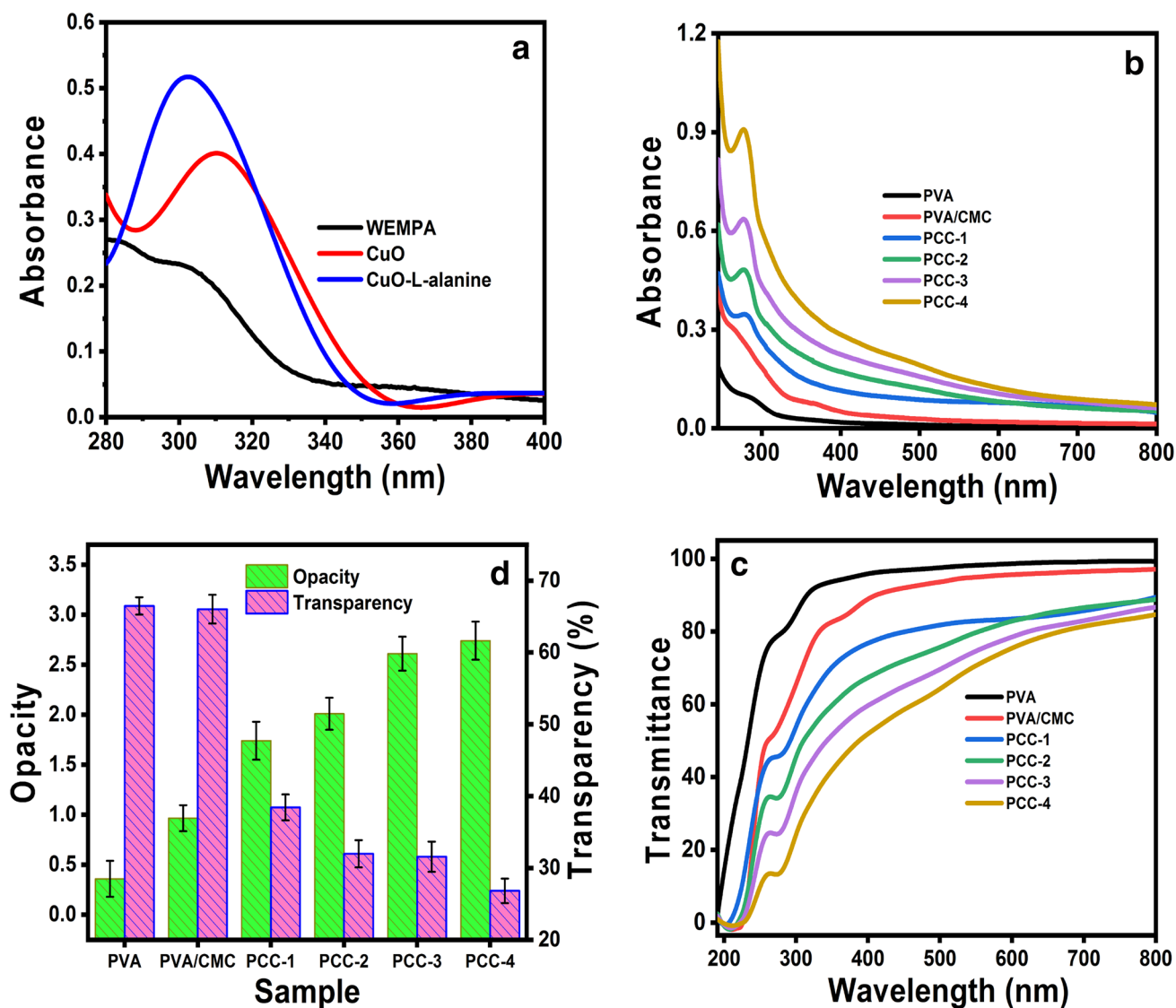
Fig. 1 a UV-Vis spectra of A: WEMPA, B: CuO nanorods and C: CuO-L-alanine; optical properties of the prepared films; b UV-Vis absorption, c % transmittance; d opacity at 500 nm and transparency at 600 nm (mean \pm SD, n=3 )
