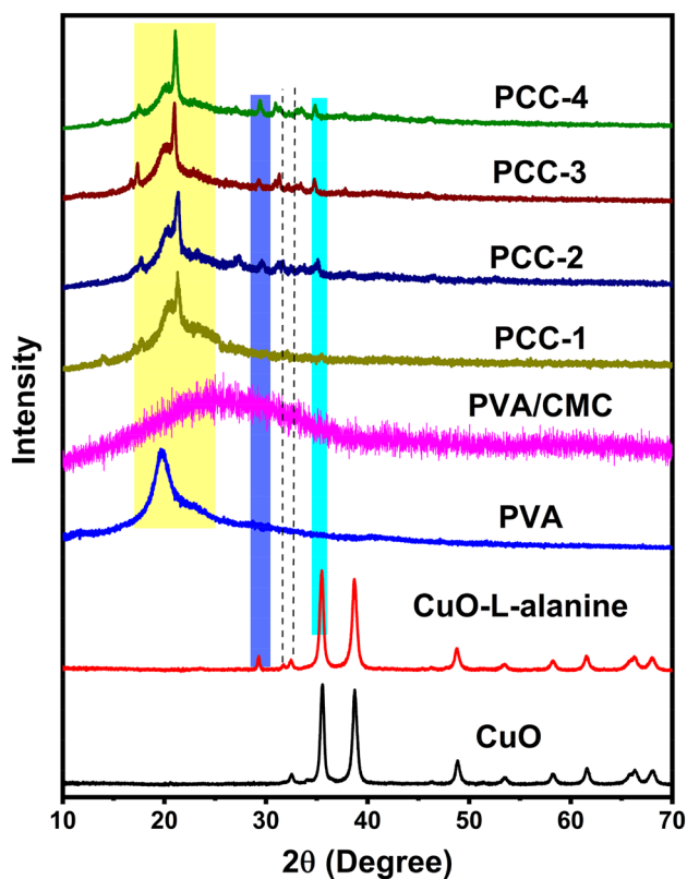
Fig. 3 XRD spectra of CuO, CuO-L-alanine, pure PVA, PVA/CMC and NC films
