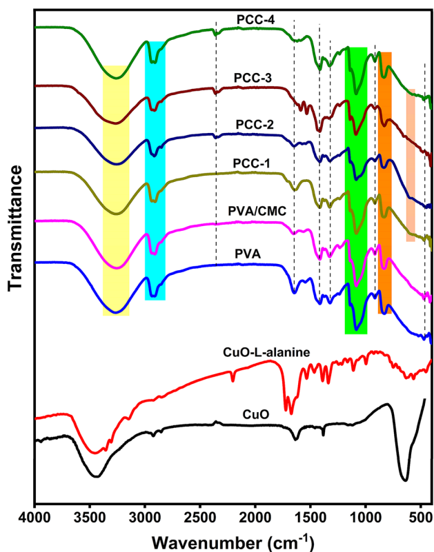
Fig. 2 FT-IR spectra of CuO, CuO-L-alanine, pure PVA, PVA/CMC and NC film
