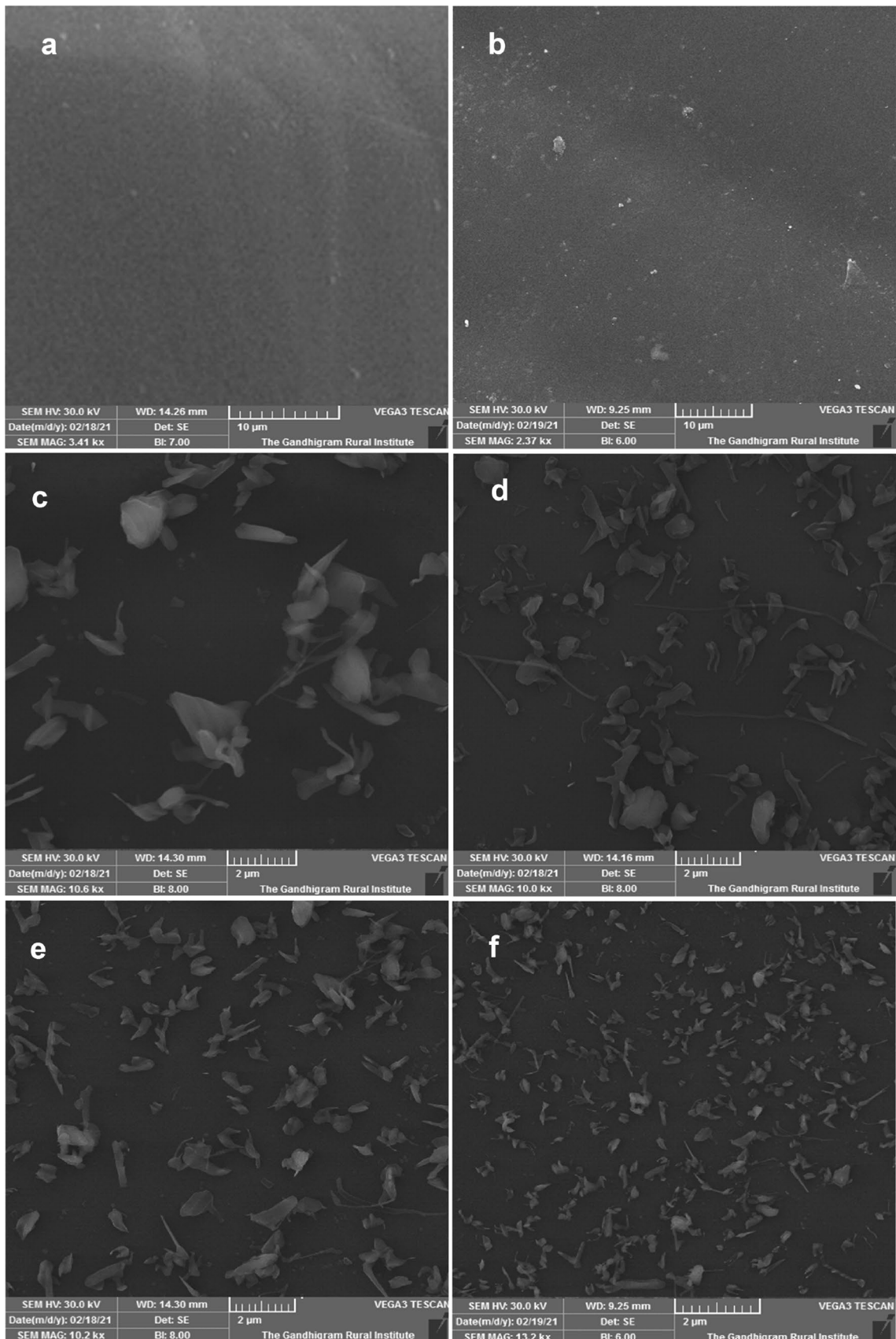
Fig. 5 SEM images of PVA (a), PVA/CMC (b), PCC-1 (c), PCC-2 (d), PCC-3 (e) and PCC-4 (f)
