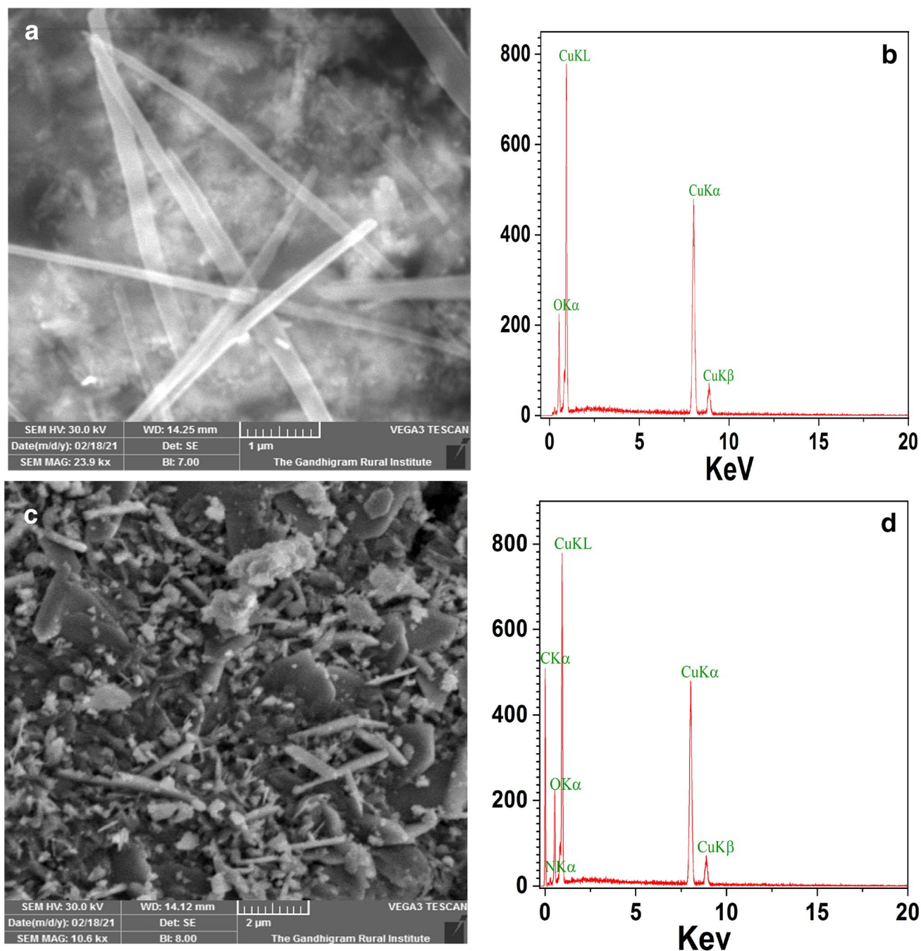
Fig. 4 SEM image of CuO (a), EDX spectrum of CuO (b), SEM image of CuO-L-alanine (c), EDX spectrum of CuO-L-alanine (d)
