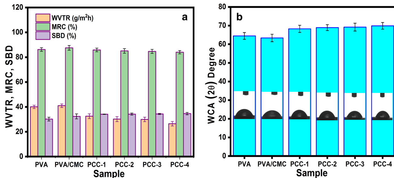
Fig. 8 WVTR, MRC and Soil burial degradation (a) and WCA (b) of PVA, PVA/CMC and NC films (mean \pm SD, n=3 )
