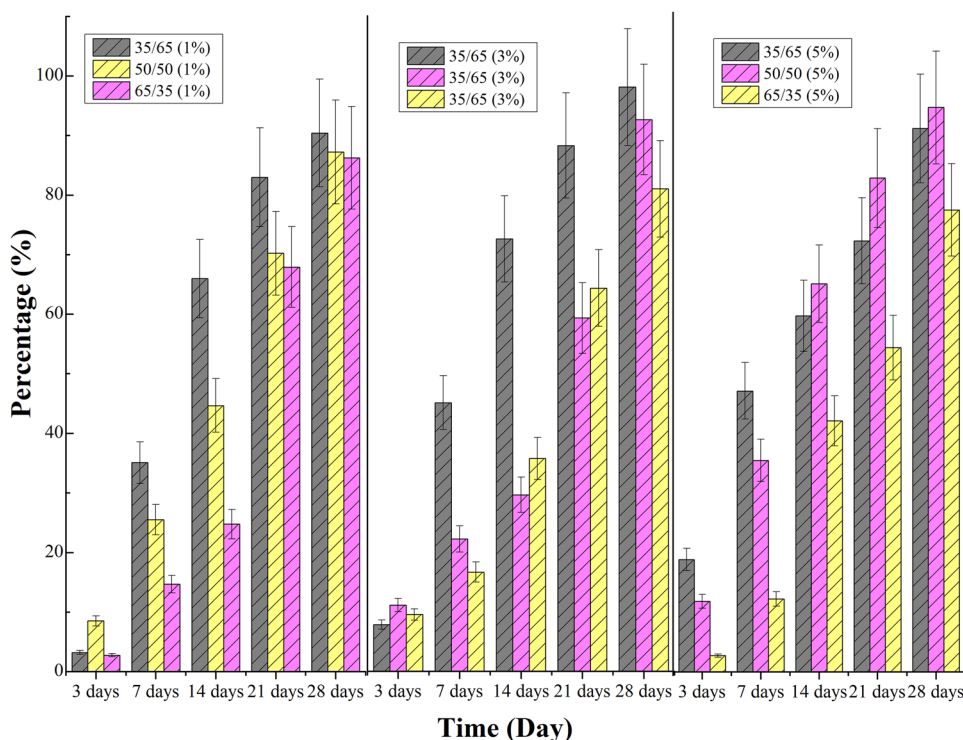
Fig. 5 Biodegradation for bioplastics composite SPF/starch/chitosan/polypropylene with different ratios of starch/chitosan and various amount of SPF in this study
