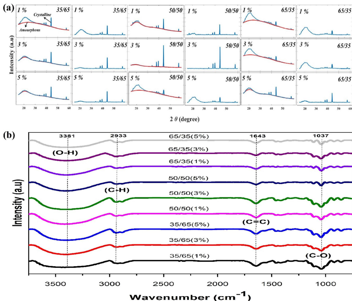
Fig. 2 X-Ray diffraction (XRD) spectra (a) and Fourier transform infrared (FTIR) spectroscopy spectra (b) of composite bio-plastic SPF/starch/chitosan/polypropylene for different ratio starch/chitosan and various amount of SPF (1%, 3%, and 5%)
