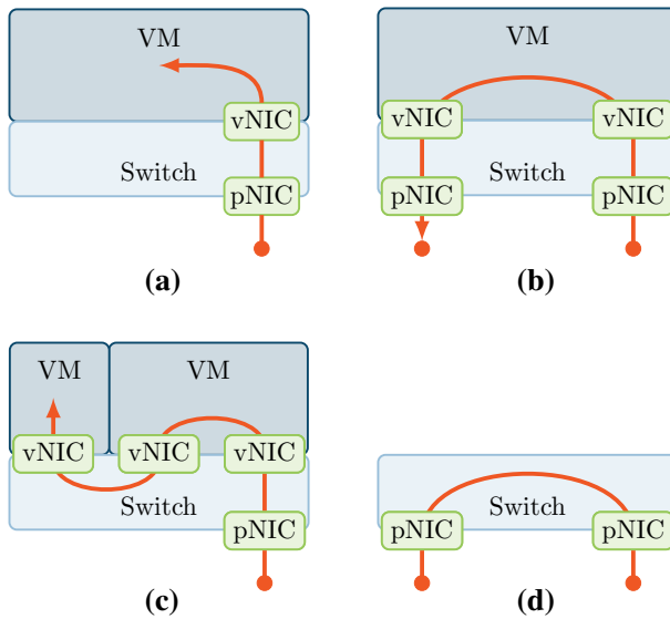
Fig. 3 Investigated test setups. a pNIC to vNIC2. b pNIC to pNIC through VM. c vNIC to vNIC. d pNIC forwarding
