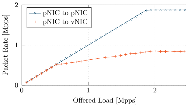
Fig. 8 Offered load versus throughput with pNICs and vNICs
