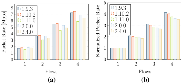
Fig. 5 Packet rate of different open vSwitch versions, 1–4 flows. a Packet rates. b Normalized to one flow
