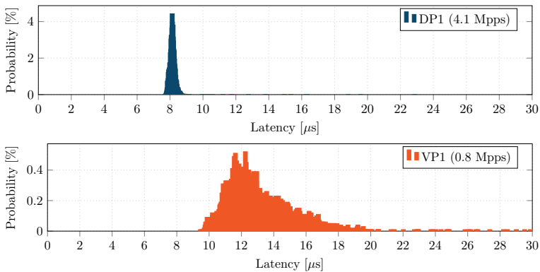
Fig. 17 Latency distribution of forwarding with DPDK
