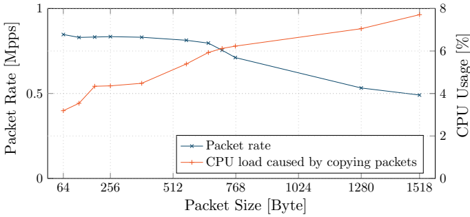
Fig. 10 Packet size versus throughput and memory copy overhead with vNICs
