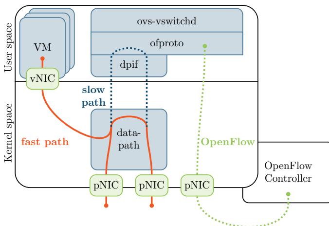
Fig. 2 Open vSwitch architecture representing the data processing flows
