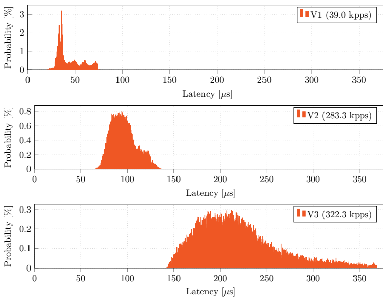
Fig. 16 Latency distribution of packet forwarding through VM
