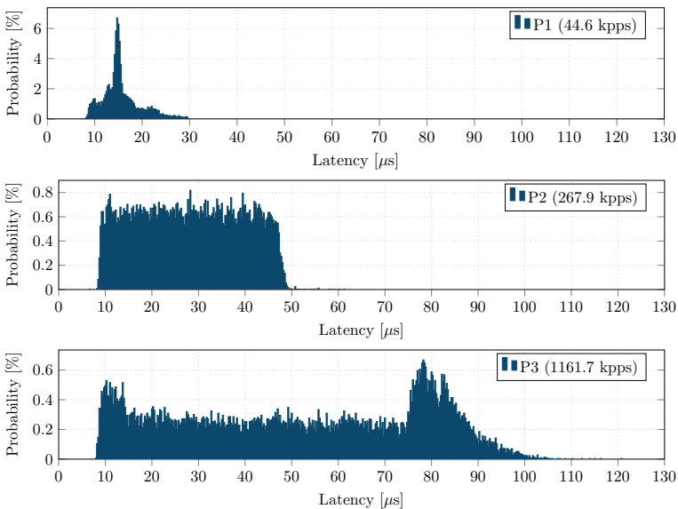
Fig. 14 Latency distribution for forwarding between pNICs
