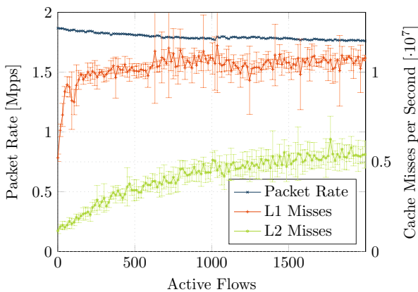
Fig. 6 Flow table entries versus cache misses
