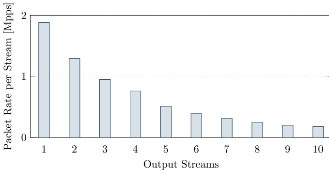
Fig. 7 Effects of cloning a flow
