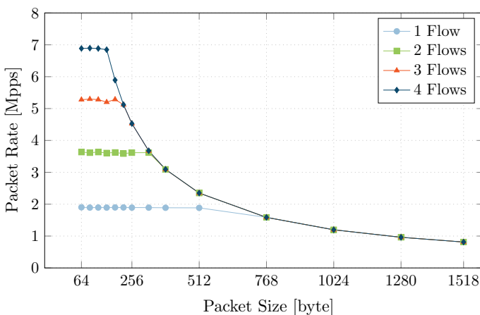
Fig. 4 Packet rate with various packet sizes and flows
