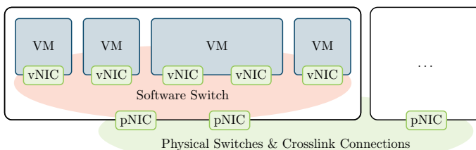
Fig. 1 Application scenario of a virtual switch
