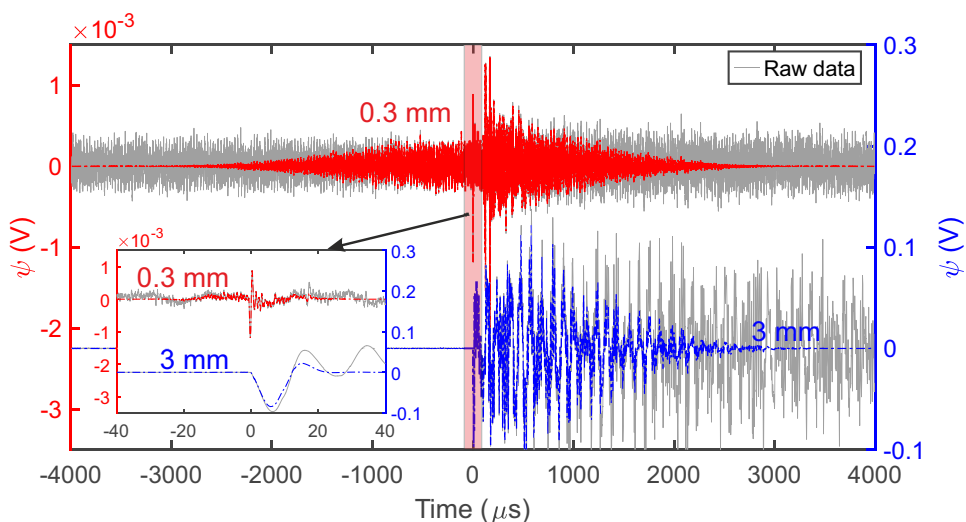
Fig. 3 Raw data (gray) and windowed data (colored) centered at the first P-wave arrival from typical acoustic events due to ball impact, with diameters of 0.3 mm (red) and 3 mm (blue), measured by the PZT sensor A1 located directly beneath the impact point. Window functions with two lengths 80 \mu s (see inset) and 8000 \mu s are used for high- and low-frequency analysis in Appendix C, respectively. (Color figure online)
