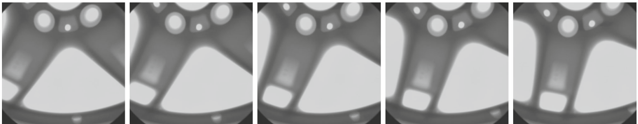
Fig. 3 Some X-ray images of an aluminum wheel (group Castings series C0001)
