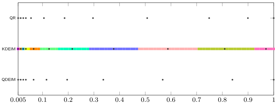
Fig. 4 Algorithm 3.2 for the Burgers' Equation with SVD, QR tolerance \epsilon_{SVD}, \epsilon_{QR} = 1 \cdot 10^{-6} . The crossmarks denote the parameters in the subsampled training set. For KDEIM each colour represents one cluster; the centroids of each of the clusters make up the subsampled training set (Color figure online)
