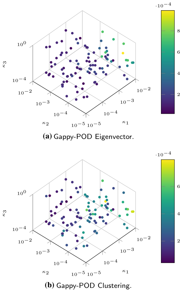
Fig. 10 Error plot for Algorithm 3.1 with coarse tolerance \text{tol}^c = 1 and subsampling based on Gappy-POD Eigenvector and Gappy-POD Clustering applied to the thermal block example. The mean error over time between the true and reduced outputs - (1/K + 1) \sum_{i=0}^K \|\mathbf{y}(\mathbf{x}(t^k, \boldsymbol{\mu})) - \tilde{\mathbf{y}}(\mathbf{z}(t^k, \boldsymbol{\mu}))\| - is plotted for all parameters in the test set
