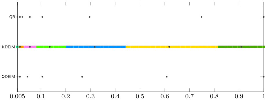
Fig. 3 Algorithm 3.2 for the Burgers' Equation with SVD, QR tolerance \epsilon_{SVD}, \epsilon_{QR} = 1 \cdot 10^{-4} . The crossmarks denote the parameters in the subsampled training set. For KDEIM each colour represents one cluster; the centroids of each of the clusters make up the subsampled training set (Color figure online)
