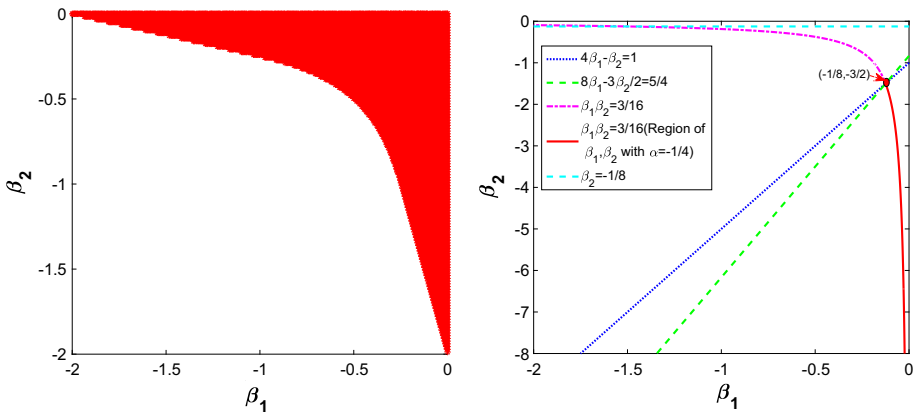
Fig. 1 The region of \beta_1, \beta_2 in the condition (4.18) for the stability. Left: \alpha = -\sqrt{\frac{1}{4} - \beta_1\beta_2} ; Right: \alpha = -\frac{1}{4}
