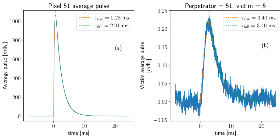
Fig. 2 a Average pulse for direct photon events in pixel 51 and b Pixel 5 average response to perpetrator pixel 51 photon events. Both measured with a Ru foil photon source. In both plots the dashed lines and legend text indicates the fitted rise and fall times for a single-exponential pulse model. These times are different for the original pulse but are nearly equal for the crosstalk response
