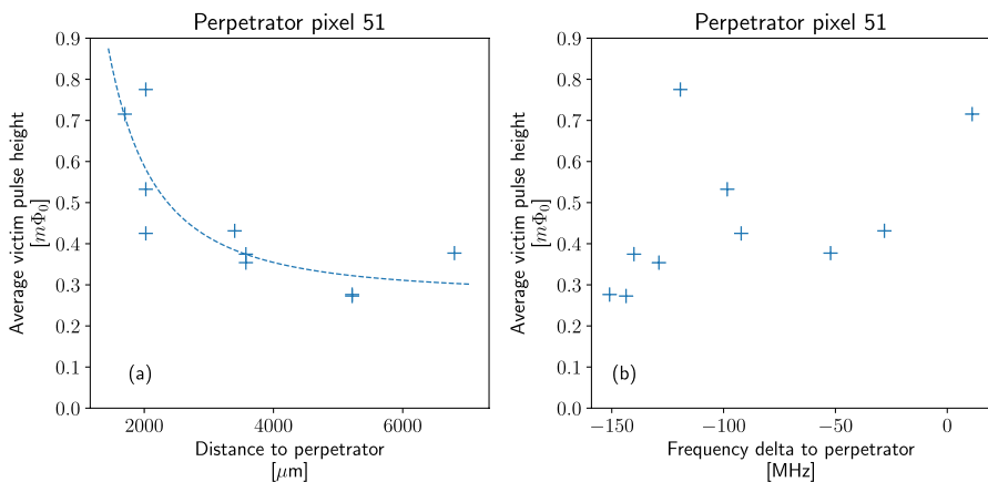
Fig. 4 a Average response magnitude as a function of physical distance between the perpetrator (pixel 51) and the victim pixels. The dashed line is 1/x^2 scaled and shifted to match the data, illustrating the expected behavior for heat flow in 2D. The measured crosstalk is in qualitative agreement with this thermal model. b Average response magnitude as a function of the difference in frequency between the perpetrator and the victim readout resonators. No significant correlation is apparent
