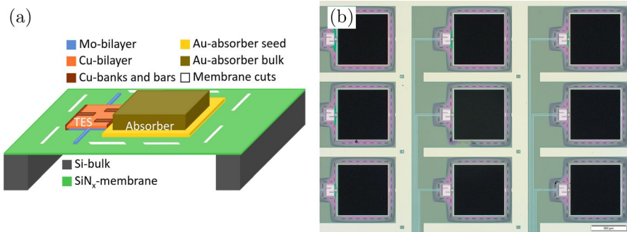
Fig. 1 a Cross-sectional schematic showing the “sidecar” design with TES and absorber on a perforated \text{SiN}_x membrane. b Optical microscope image showing a 3 \times 3 pixel section of a completed array of this design, fabricated at ANL
