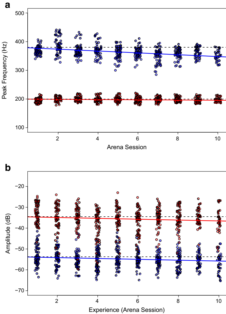
Fig. 1 Relationship between a frequency and b amplitude of buzzes with accumulating experience. Points represent the raw data and solid lines represent regression lines for flight ( red ) and sonication ( blue ) buzzes obtained from the statistical analysis, and omitting non-significant interaction terms. Broken lines represent the intercept value for each buzz type. Horizontal jitter has been applied to facilitate interpretation of the figure
