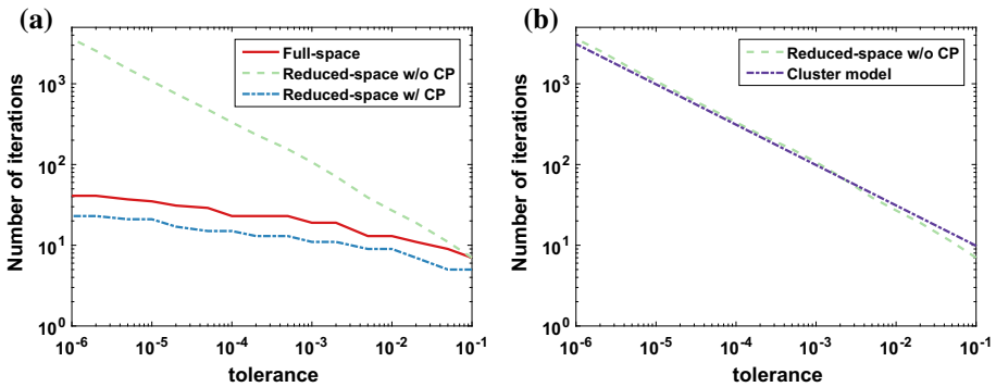
Fig. 2 (a) Comparison of the number of branch-and-bound iterations between the full-space and reduced-space convex relaxation-based lower bounding schemes considered in this work for different absolute termination tolerances for Example 18. The solid line indicates the number of iterations of the convex relaxation-based full-space lower bounding scheme, the dashed line indicates the number of iterations of the convex relaxation-based reduced-space lower bounding scheme without constraint propagation, and the dash-dotted line indicates the number of iterations of the convex relaxation-based reduced-space lower bounding scheme with constraint propagation. (b) Comparison of the number of branch-and-bound iterations of the convex relaxation-based reduced-space lower bounding scheme without constraint propagation with the predictions from the cluster problem model for different absolute termination tolerances for Example 18. The dashed line indicates the number of iterations of the convex relaxation-based reduced-space lower bounding scheme without constraint propagation, and the dash-dotted line indicates the predicted number of iterations from the cluster problem model
