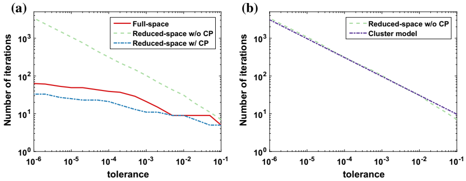
Fig. 1 (a) Comparison of the number of branch-and-bound iterations between the different lower bounding schemes considered in this work for different absolute termination tolerances for Example 16. The solid line indicates the number of iterations of the full-space lower bounding schemes, the dashed line indicates the number of iterations of the reduced-space lower bounding schemes without constraint propagation, and the dash-dotted line indicates the number of iterations of the reduced-space lower bounding schemes with constraint propagation. (b) Comparison of the number of branch-and-bound iterations of the reduced-space lower bounding schemes without constraint propagation with the predictions from the cluster problem model for different absolute termination tolerances for Example 16. The dashed line indicates the number of iterations of the reduced-space lower bounding schemes without constraint propagation, and the dash-dotted line indicates the predicted number of iterations from the cluster problem model
