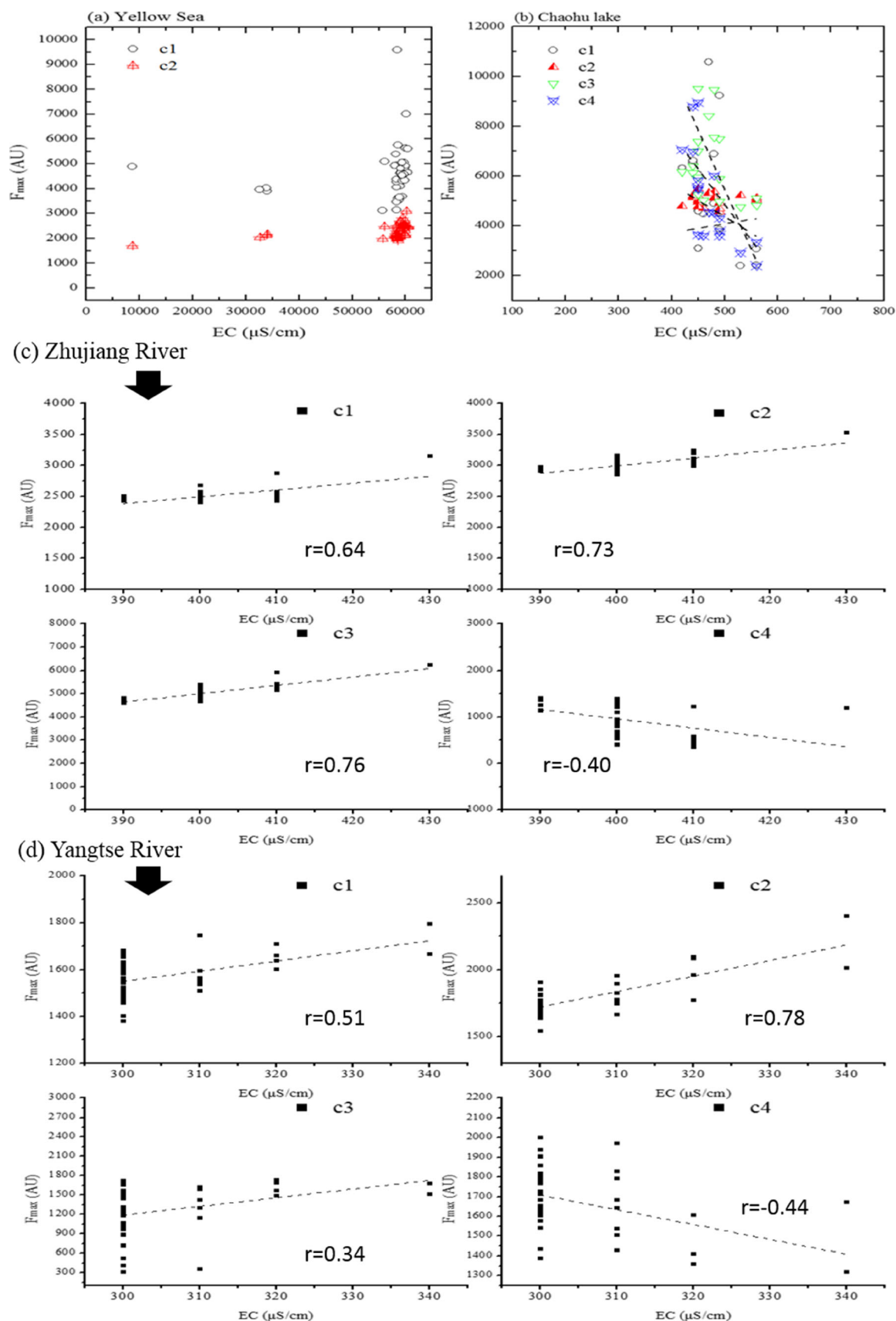
Fig. 7 Results of EC vs. F_{\max} of EEMs-PARAFAC components of (a) Yellow Sea (b) Chaohu lake (c) Zhujiang River, and (d) Yangtse River. A similar correlation characteristics of EC and fluorescence components were also found in other natural water
