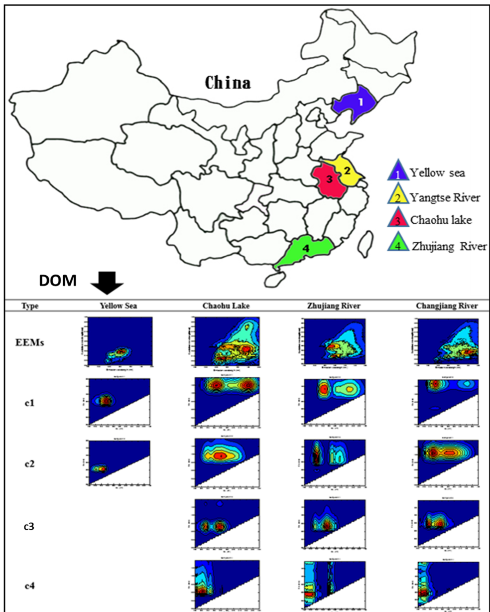
Fig. 6 Sampling locations in China's province map and the EEMs-PARAFAC components of DOM in these water environments. In the plots of EEMs and components, x-axes stand for the emission wavelength ( E_m ) and excitation wavelength ( E_x ), respectively, while y- axes stand for excitation wavelength ( E_x ) and emission wavelength ( E_m ), respectively
