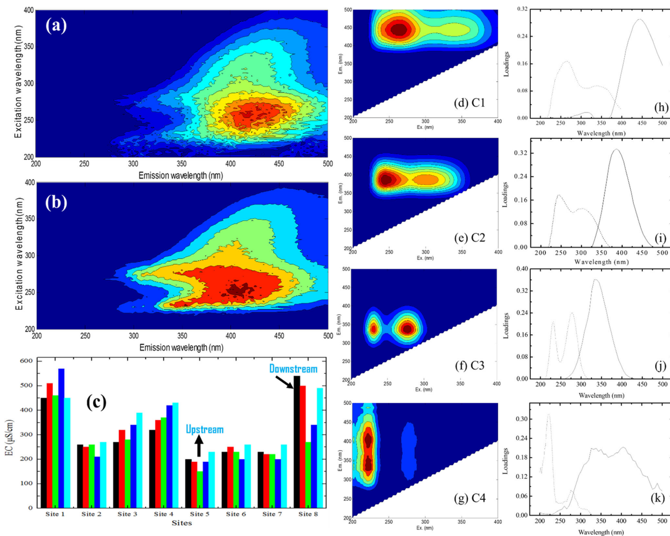
Fig. 3 Results of three dimension excitation-emission matrix spectroscopy of DOM: (a) DOM of upstream river site 8, (b) DOM of downstream site 5, and (c) EC distribution of all sample sites after measuring five times during 2018–2019 year. The Roman numeral colors represent five categories of EEM data: I) aromatic protein-like materials, II) aromatic protein-like materials, III) fulvic acid-like materials, IV) soluble microbial metabolites, and V) humic substance-like materials. Signatures of four
