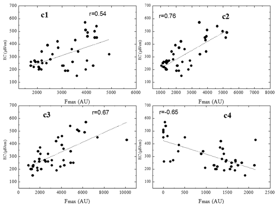
Fig. 4 Results of plots of EC vs. EEMs-PARAFAC model components of dissolved organic matter samples. The results showed that three components were positive correlation with EC and one component was
