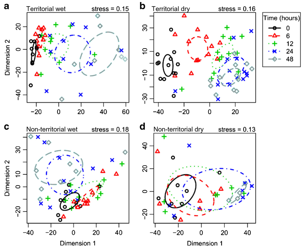
Fig. 1 Multidimensional scaling (MDS) plot based on Bray-Curtis similarities of the variation of VOCs emitted from territorial male dung over 48 hr during, (a) wet and (b) dry seasons, and from non-territorial male dung over 48 hr during (c) wet and (d) dry seasons. Encompassing circles represent 95% confidence intervals
