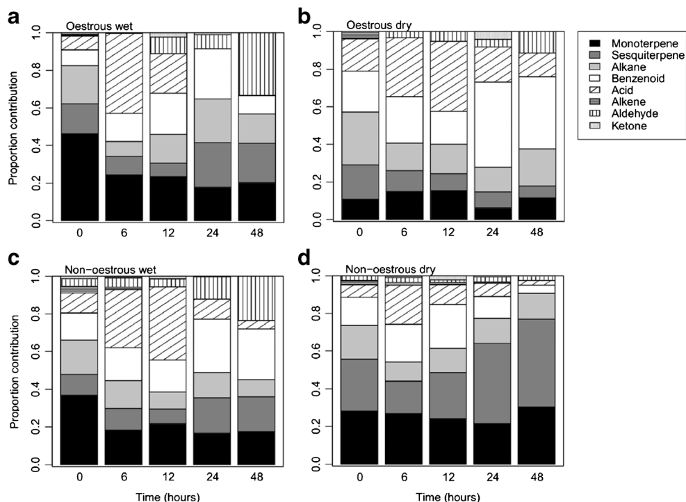
Fig. 4 Odour composition of oestrous female dung over 48 hr during, the (a) wet and (b) dry seasons, and non-oestrous female dung over 48 hr during, the (c) wet and (d) dry seasons
