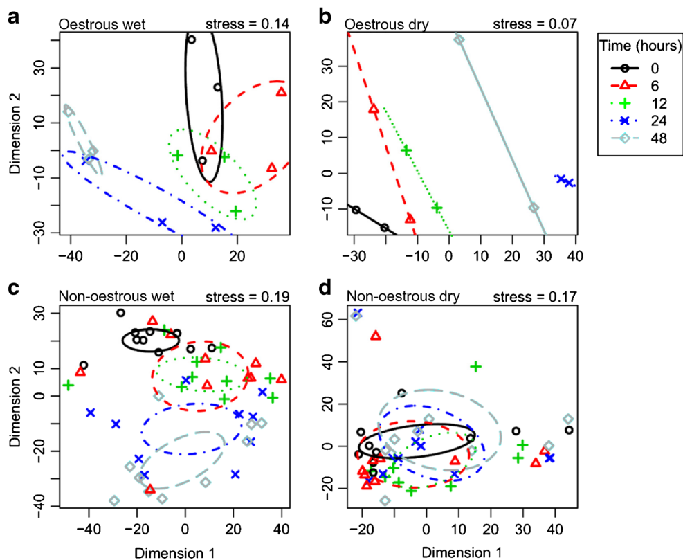
Fig. 2 Multidimensional scaling (MDS) plot based on Bray-Curtis similarities of the variation of VOCs emitted from oestrous female dung over 48 hr during, (a) wet and (b) dry seasons, and from non-oestrous female dung over 48 hr during, (c) wet and (d) dry seasons. Encompassing circles represent 95% confidence intervals
