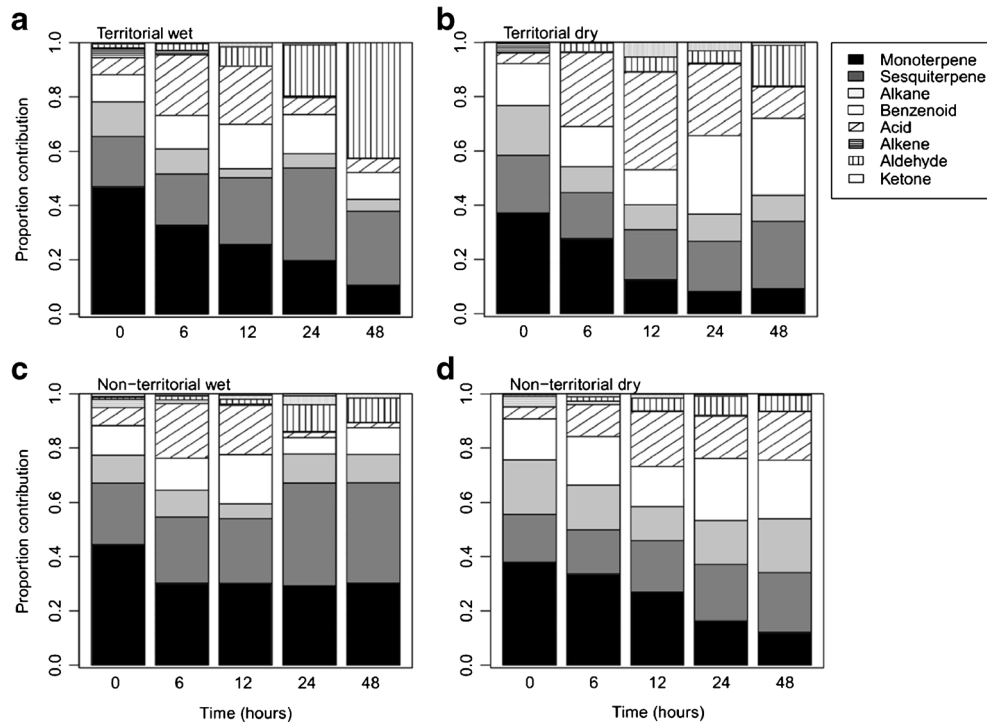
Fig. 3 Odour composition of territorial male dung over 48 hr during, the (a) wet and (b) dry seasons, and non-territorial male dung over 48 hr during, the (c) wet and (d) dry seasons
