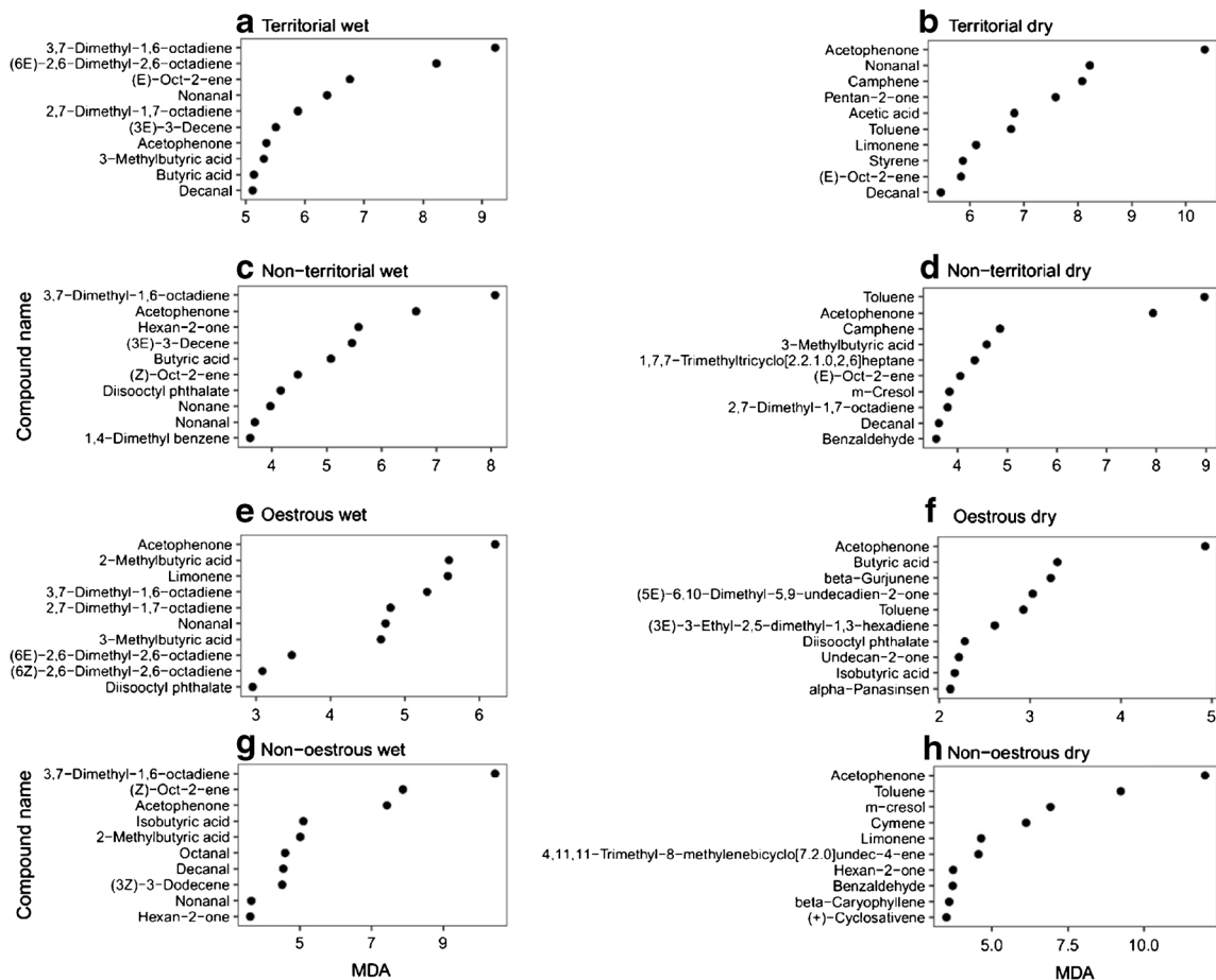
Fig. 5 The importance of volatile organic compounds (VOCs) for distinguishing the age of dung from territorial males, a ) wet season, b ) dry season; non-territorial males c ) wet season, d ) dry season; oestrous
