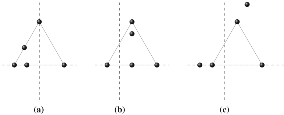
Fig. 1 Three different configurations in the five-body problem where after removing two bodies, one equilateral triangular configuration and two collinear configurations are obtained. All three are discarded by the perpendicular bisector theorem to be central configurations in the five-body problem
