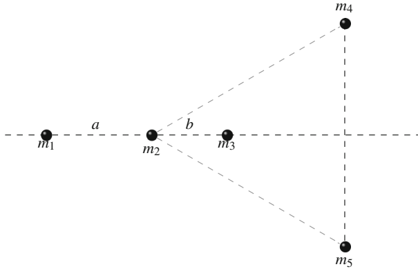
Fig. 2 Euler plus Lagrange stacked central configuration in the planar five-body problem
