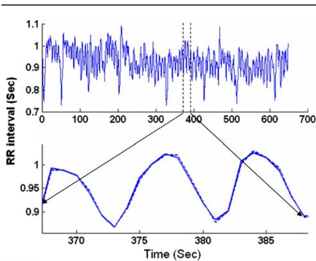
Fig. 3. Comparison of the HRV and PPG signals in the top panel shows that the signals are nearly identical. The bottom panel shows a segment of the upper panel, which further illustrates the closeness of the two signals.
