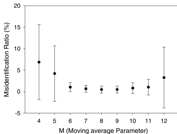
Fig. 4. Incorrect identification ratio of the PPG as a function of the size of the moving average parameter. Note that the incorrect identification ratio is relatively low when M is between f_s/6 and f_s/9 .
