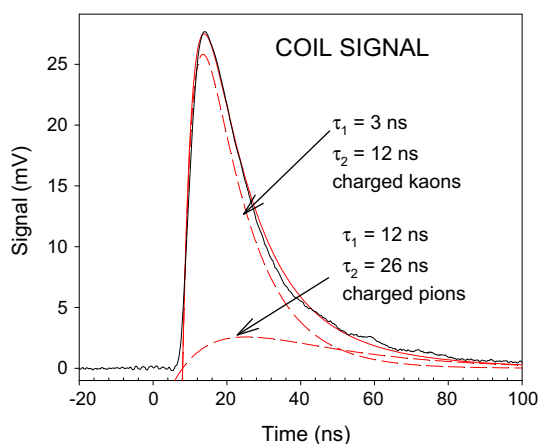
Fig. 7 Current coil signal with D(0) on target. Coil at position of inner collector in Fig. 2. Note that the pions \pi^\pm have rise time of 12 ns equal to the decay time of the kaons K^\pm as required for the decay chain K^\pm \rightarrow \pi^\pm \rightarrow \mu^\pm . The actual particle current is probably due to muons
