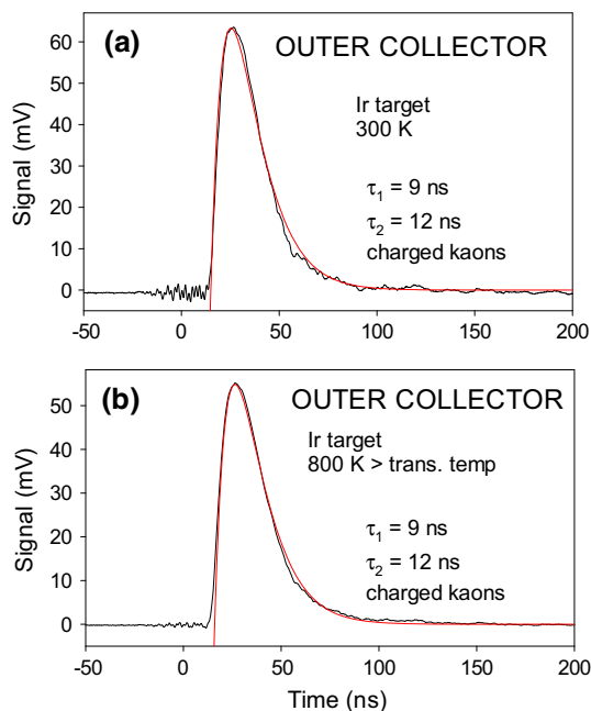
Fig. 5 Charged kaon signal at the outer collector in Fig. 2 with bias -24 \text{ V} . The meson signal exists even at a temperature of 800 K, above the D(0) on Ir transition temperature of 525 K [28]
