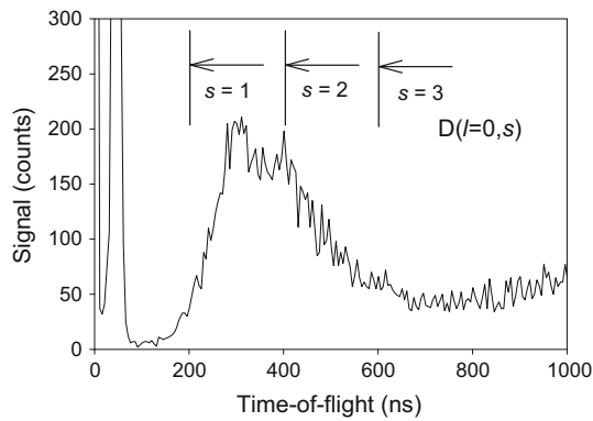
Fig. 4 Sum of all the TOF spectra in Fig. 3, showing that the distribution peaking at 300–400 ns contains a large contribution from the lowest level s = 1 in which nuclear processes are expected
