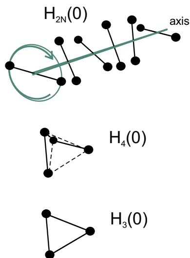
Fig. 1 Shape of the chain or “bead” clusters H_{2N}(0) forming the superfluid phase H(0) and non-superfluid cluster types H_3(0) and H_4(0)
