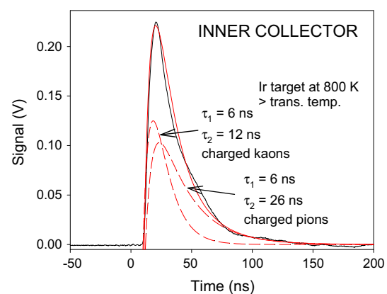
Fig. 6 Combined charged kaon and pion signal at the inner collector in Fig. 2 with bias -24 \text{ V} . The meson signal exists even at a temperature of 800 K, above the D(0) on Ir transition temperature of 525 K [28]
