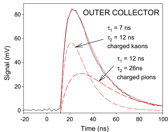
Fig. 8 Signal at outer collector with bias -24 V with the coil in the beam in the same experiment as in Fig. 7. Note that the pions \pi^\pm have rise time of 12 ns equal to the decay time of the kaons K^\pm as required for the decay chain K^\pm \rightarrow \pi^\pm \rightarrow \mu^\pm . The actual signal is probably due to muons giving secondary electron ejection at collector
