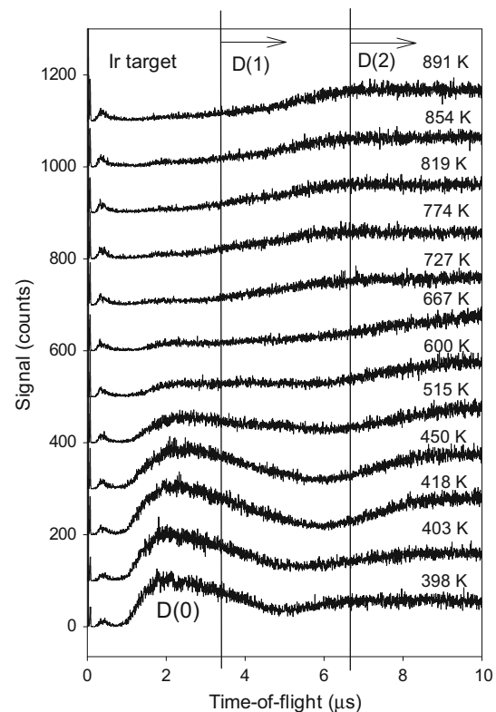
Fig. 3 TOF spectra at 45° detector position relative to laser beam. D(0) on Ir surface. Temperature variation shown
