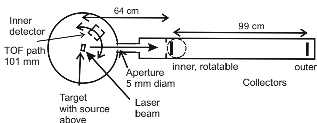
Fig. 2 Horizontal cut through the apparatus
