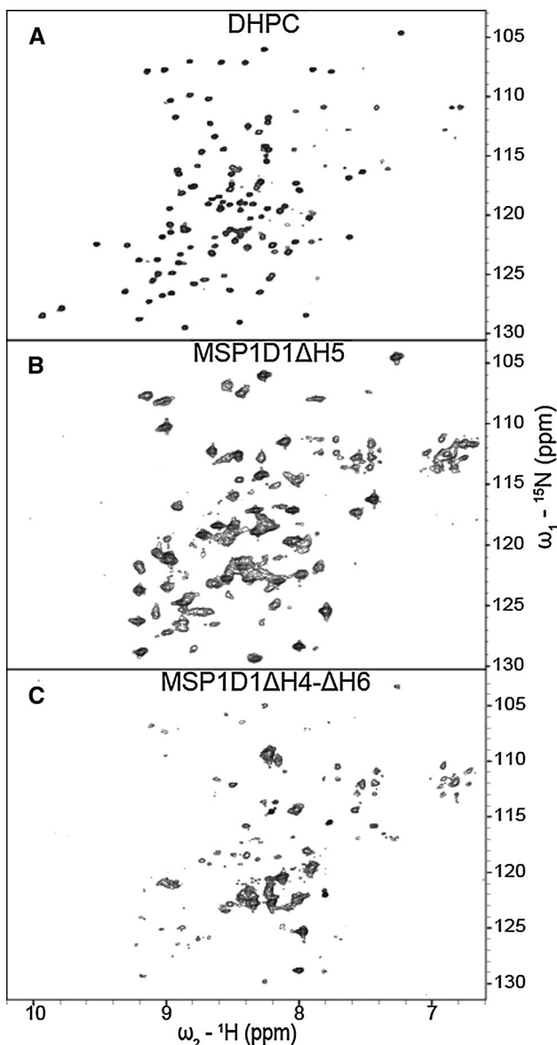
Fig. 6 ^{15}\text{N} - ^1\text{H} TROSY spectra of ^2\text{H} -, ^{15}\text{N} -labeled OprH \Delta L1 \Delta L4 in DHPC micelles and in MSP nanodiscs of different sizes. The OprH \Delta L1 \Delta L4 samples are in a DHPC micelles, b MSP1D1 \Delta H5, and c MSP1D1 \Delta H4- \Delta H6. All spectra were collected at 800 MHz and 45 °C
