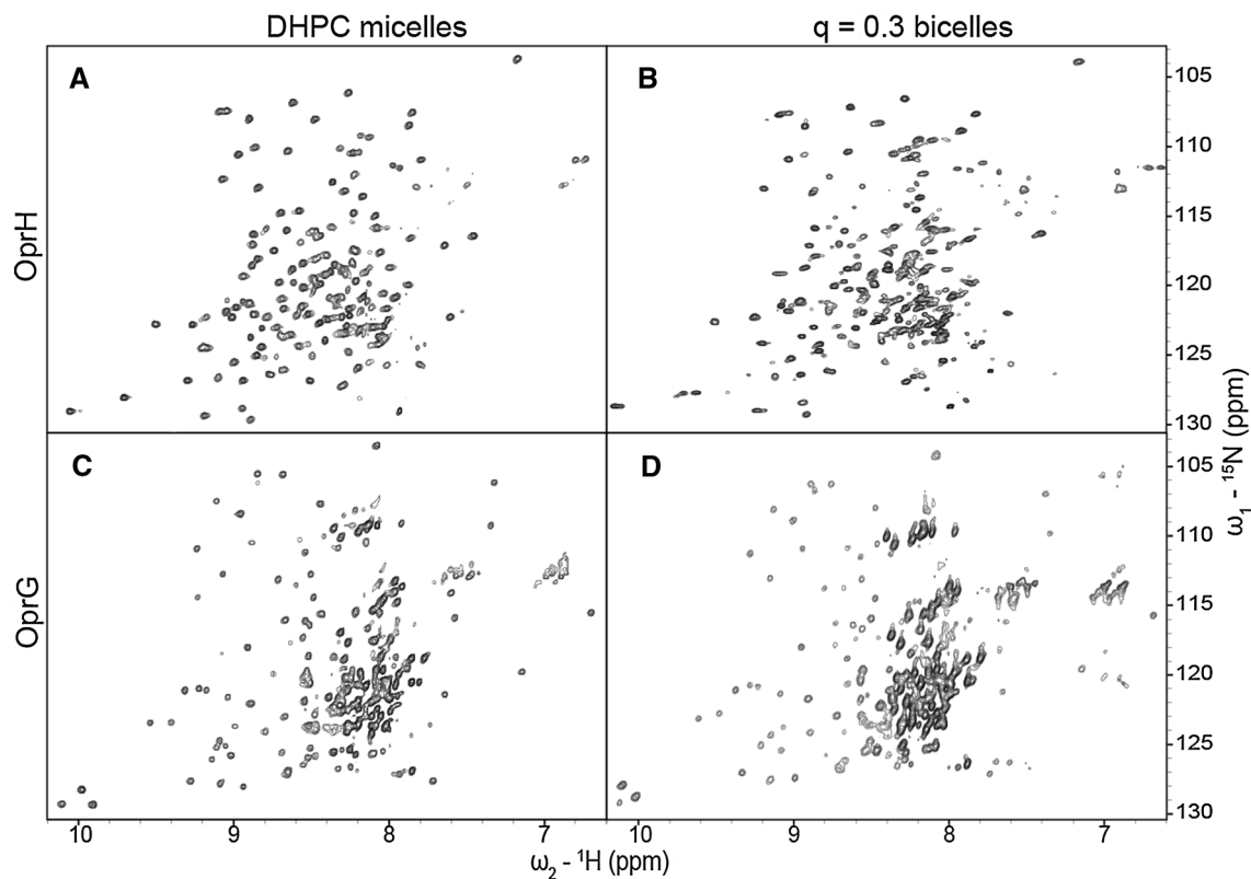
Fig. 7 ^{15}\text{N} - ^1\text{H} TROSY spectra of ^2\text{H} -, ^{13}\text{C} -, ^{15}\text{N} -labeled OprH ( a and b ) and OprG ( c and d ) in DHPC micelles ( a and c ) and in q = 0.3 DHPC:DMPC:DHPS:DMPS (27:9:3:1) bicelles ( b and d ). All spectra were collected at 800 MHz and 45 °C
