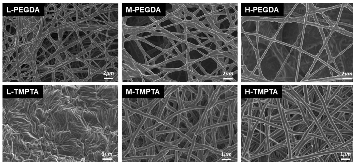
Figure 7 FE-SEM images of the photo-cured electrospun fibrous membranes of PEO/PEGDA and PEO/TMPTA after water treatment.
