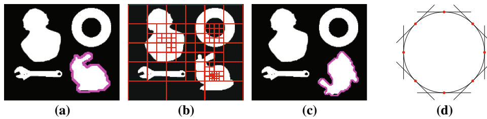
Fig. 4 Shape location with branch and bound. We are searching for a bunny among a collection of other shapes via branch and bound. a Illustration of c_{\mathcal{F}}(f_x, f_y) , white indicating foreground affinity. The optimal segmentation is given by the purple line. b The covering set L (4.10) upon convergence of branch and bound, projected onto the two translation components, shown relative to the query image. Very dissimilar shapes such as the wrench can be ruled out at a coarse level while more
