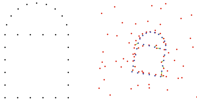
Fig. 16 Segmenting and matching on point clouds. Left : the template, a schematic ‘gate’. Right : the original shape is subjected to perspective transformations (foreshortening, rotation, scale), noise and additional, noisy observations are added. With branch and bound the original shape is detected. This could be applied to matching sparse interest points on images (Color figure online)
