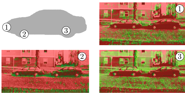
Fig. 13 Inhomogeneous appearance model. For each template pixel a local appearance model was learned. Top left : template X with three selected (super-)pixels \{x_i\}_i . Top right, bottom row : costs c_{\mathcal{F}}(x_i, \cdot) for the three selected pixels. The appearance cost of single pixels is not very informative. Only by combining costs from all template pixels and their relative spatial position enables one to find the objects (Fig. 14) (Color figure online)
