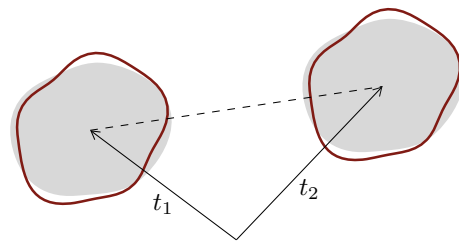
Fig. 2 Explicit transformation variables and non-convexity. Gray shading indicates ‘foreground features’. Placing the template (red contour) at t_1 or t_2 yields equally good hypotheses. Were the prior functional convex in the translation variable, any point along the line (1 - \alpha) \cdot t_1 + \alpha \cdot t_2 for \alpha \in [0, 1] would yield an at least equally good proposal, which is clearly unreasonable (Color figure online)
