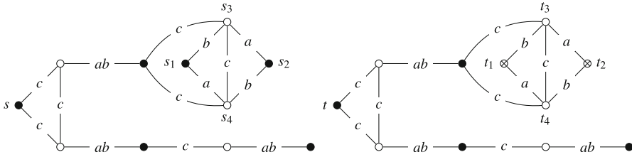
Fig. 8 Models M_s (left) and N_t (right). Propositional variable p is true in black and crossed-out states, and q is true in crossed-out states
