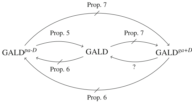
Fig. 10 Relative expressivity of GALD^{pa-D} , GALD , and GALD^{ga+D} . An arrow from one logic to another signifies that the latter is at least as expressive as the former, striked out arrow—not at least as expressive, and the arrow with the question mark represents an open problem
