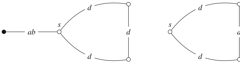
Fig. 4 Submodels, N (left) and O (right), of model M
