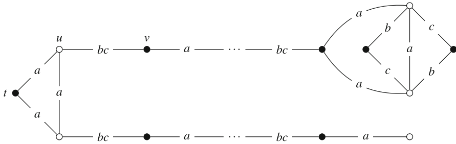
Fig. 6 Model N_t . Propositional variable p holds in black states
