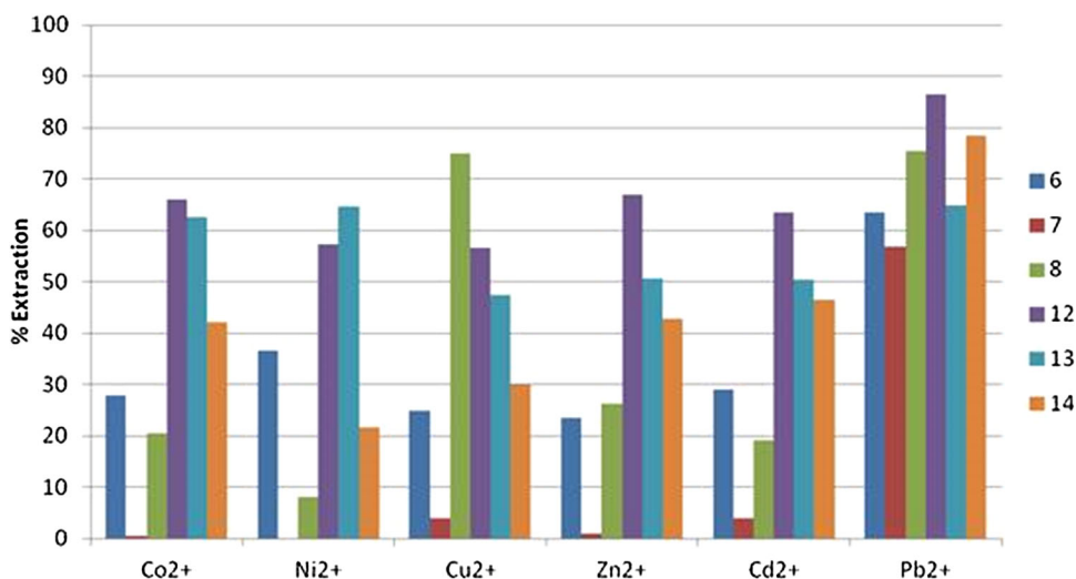
Fig. 4 Trend in % extraction by metal ion for all host compounds 6–8 and 12–14
