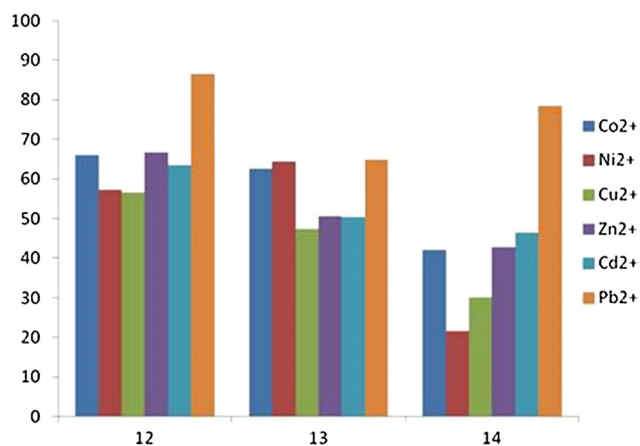
Fig. 3 % Extraction of the heavy metal divalent ion picrate salts from aqueous solution into dichloromethane by spirolactam-calix[4]-arene host compounds 12–14 , with lower rim methoxy groups
