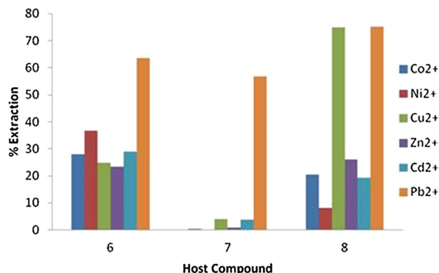
Fig. 2 % Extraction of the heavy metal divalent ion picrate salts from aqueous solution into dichloromethane by spirolactam-calix[4]arene host compounds 6–8 , with lower rim phenolic groups
