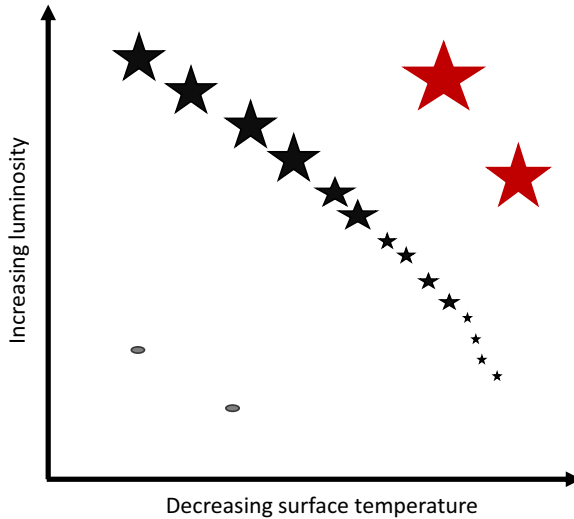
Fig. 1 Schematic H–R diagram
