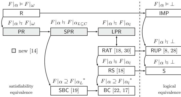
Fig. 1 Landscape of redundancy notions of non-empty clauses. R denotes all redundant clauses and IMP stands for implied clauses. A path from X to Y indicates that X is more general than Y. The asterisk (*) denotes that the exact characterization implies the shown one, e.g., for every set-blocked clause, the property F|\alpha \supseteq F|\alpha_L holds, but not vice versa
