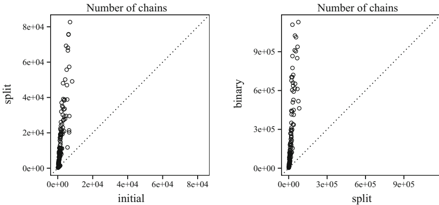
Fig. 13 Number of chains before and after splitting; binary resolution steps
