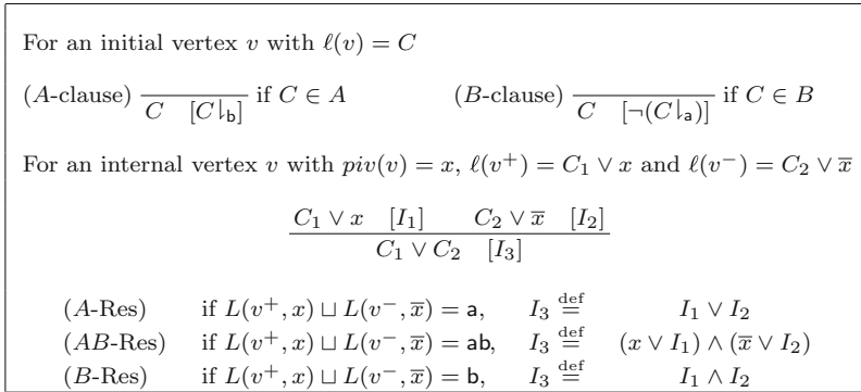
Fig. 2 Labelled interpolation system for resolution proofs
