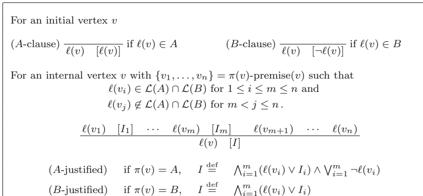
Fig. 20 Interpolation system \text{ltp}_{KV} for local proofs
