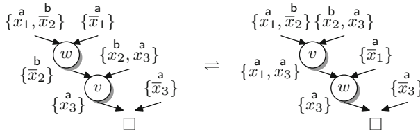
Fig. 8 Reordering resolution chains
