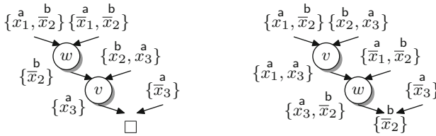
Fig. 9 Reordering in the presence of merge literals may invalidate the resolution chain
