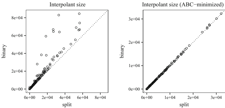
Fig. 18 Size of AIG circuit; before and after reduction by ABC
