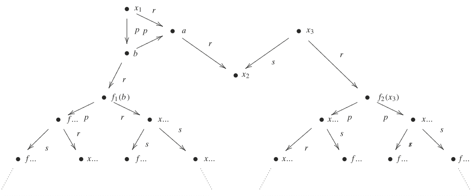
Fig. 4 An \mathcal{ALC} -admissible graph associated with an abductive proof: every Skolem vertex has exactly one predecessor and can be only succeeded by a tree-shaped subgraph containing no individual names
