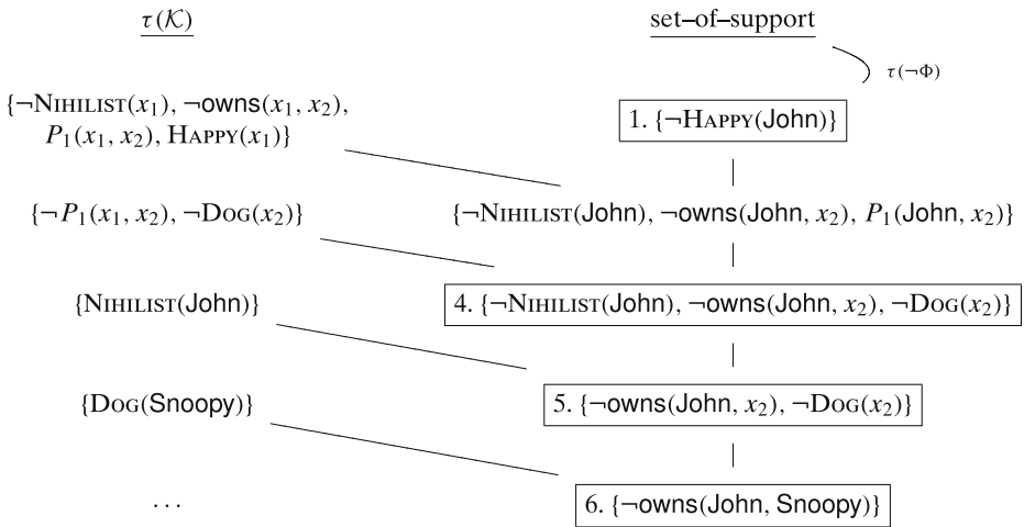
Fig. 6 Happy John problem: resolution proofs
