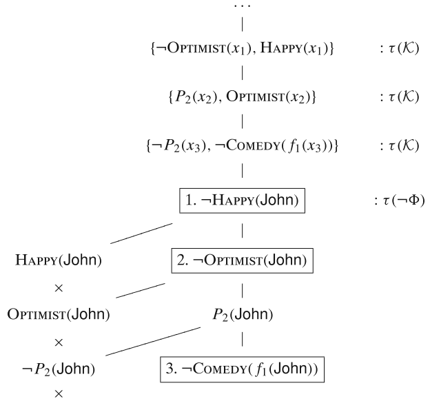
Fig. 5 Happy John problem: tableaux proofs
